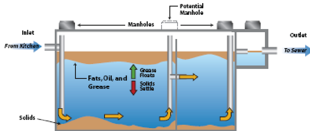
CONVENTIONAL GREASE INTERCEPTOR Outdoor, In-ground-Precast Concrete (Typical)
