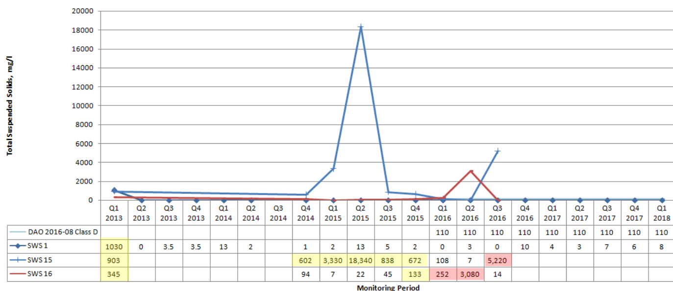
Figure 6-65: Plot of TSS monitoring data for surface water bodies upstream of the Project (SW1, SW15, and SW16)
