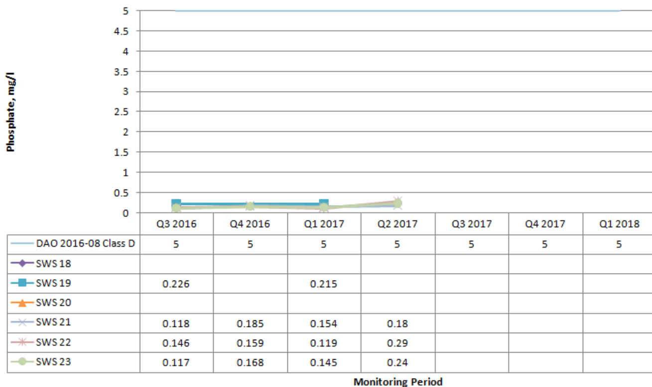
Figure 6-64: Plot of Phosphate monitoring data for ambient water quality monitoring stations located downstream and outside the Project area (SWS 18 – SWS 23)
