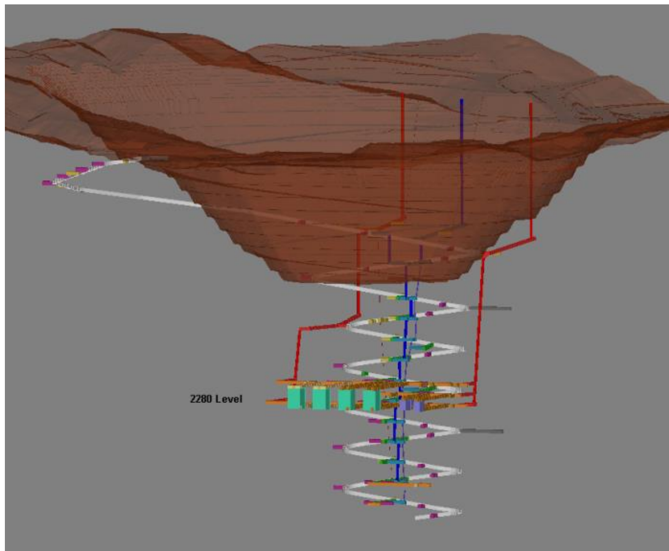
Figure 1-13: Extent of mine development at the onset of production, 2280 Level
