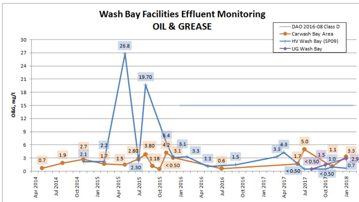
Figure 6-27: Wash Bay Facilities Effluent Monitoring Trend for O&amp;G (Carwash Bay, HV Wash Bay, UG Wash Bay)
