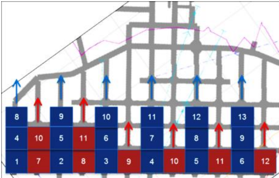
Figure 1-18: Conceptual primary-secondary stopping sequence
