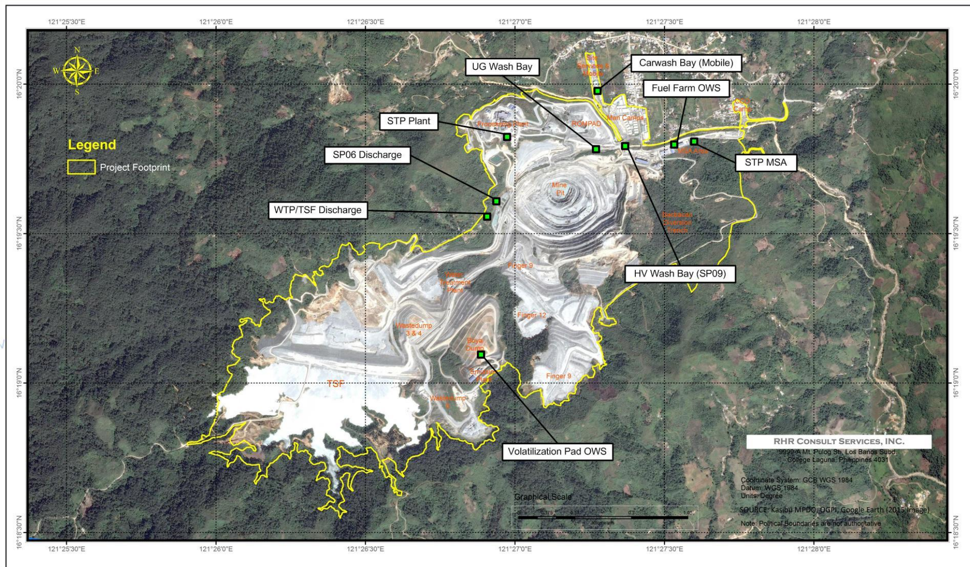
Figure 2-36: OGPI Effluent Discharge Map
