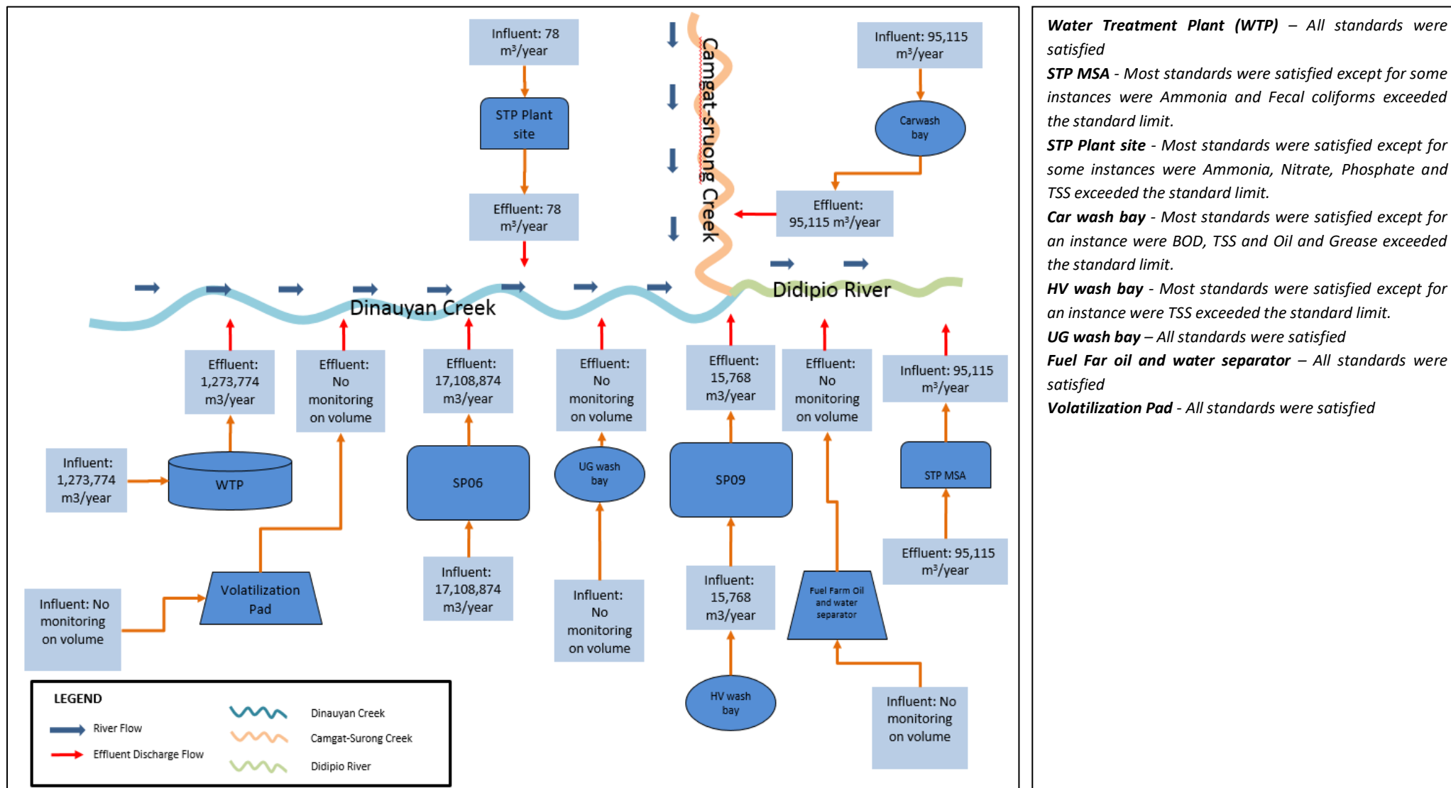
Figure 2-35: Effluent Discharge Block Diagram
