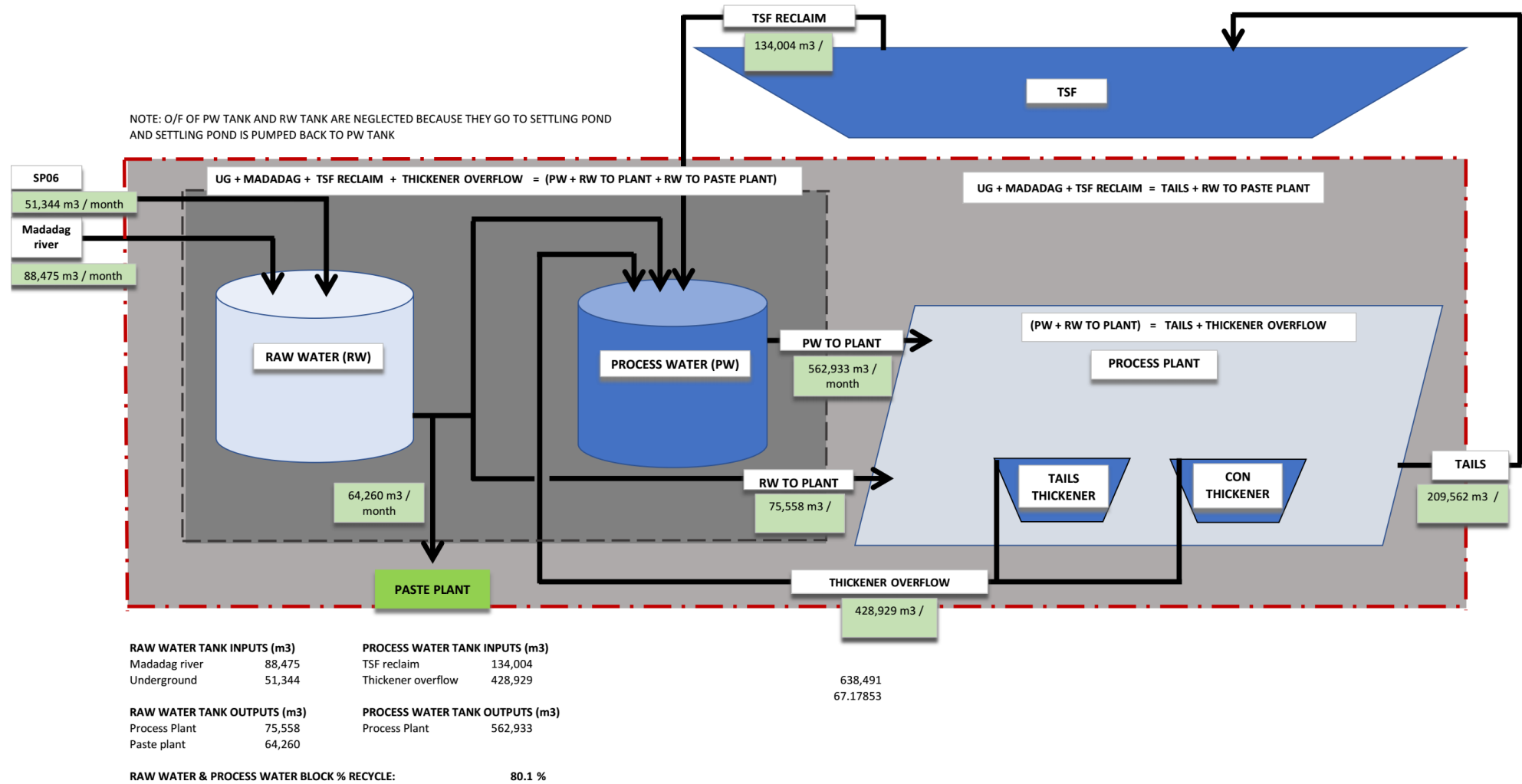
Figure 1-6: Water Balance for 4.3 Mtpa
