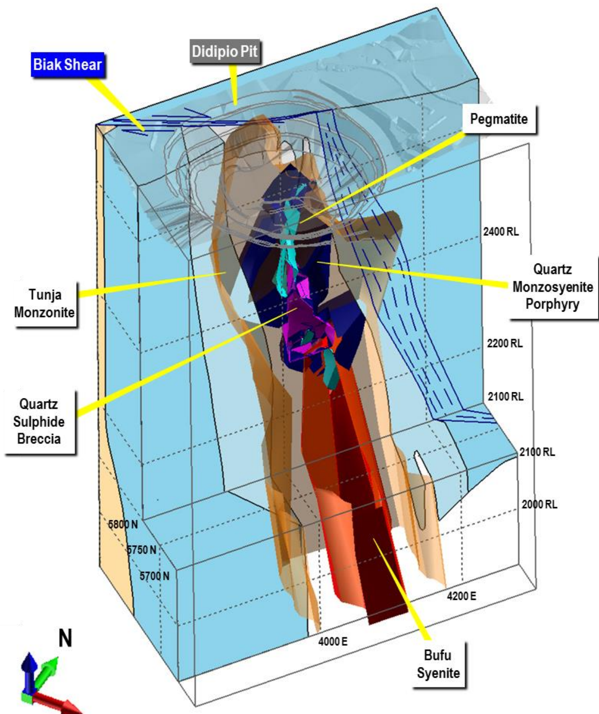
Figure 2-10: Didipio Operation Geology Cut Out as of September 30, 2014 Source: Technical Report for the Didipio Gold/Copper Operation, Griffiths et. al., 2014
