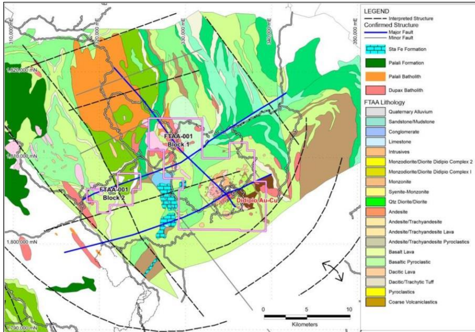
Figure 2-7: Regional Geology
