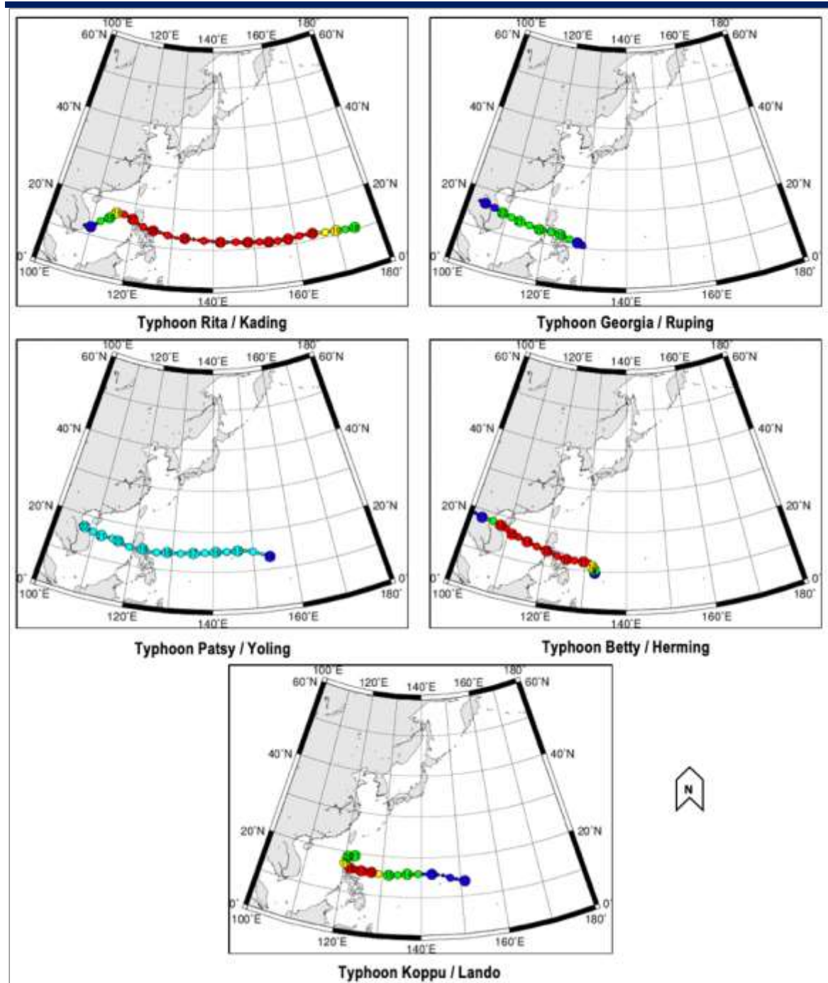
Figure 2.2-46 Individual Tracks of Top 5 Typhoons
