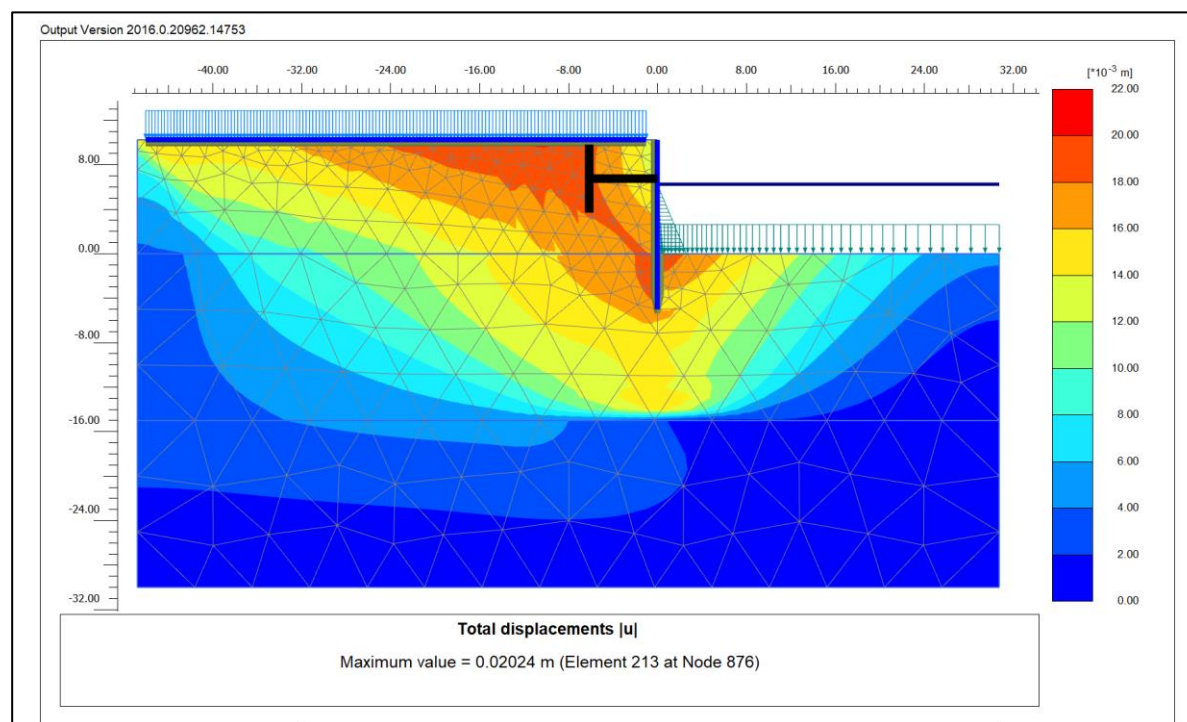
Figure 2.1-43 Plaxis Result – Total Displacement (Island A)
