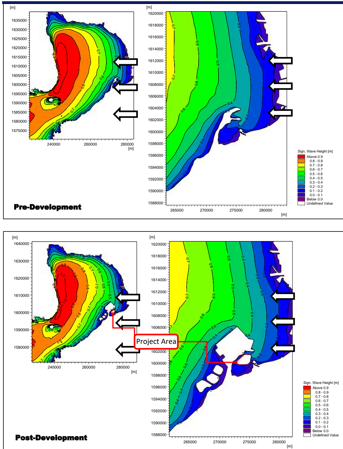
Figure 2.2-59 Wave Climate due to 5-8 mps Surface Winds & Offshore Waves from E at MHHW (Pre- & Post-Devt)
