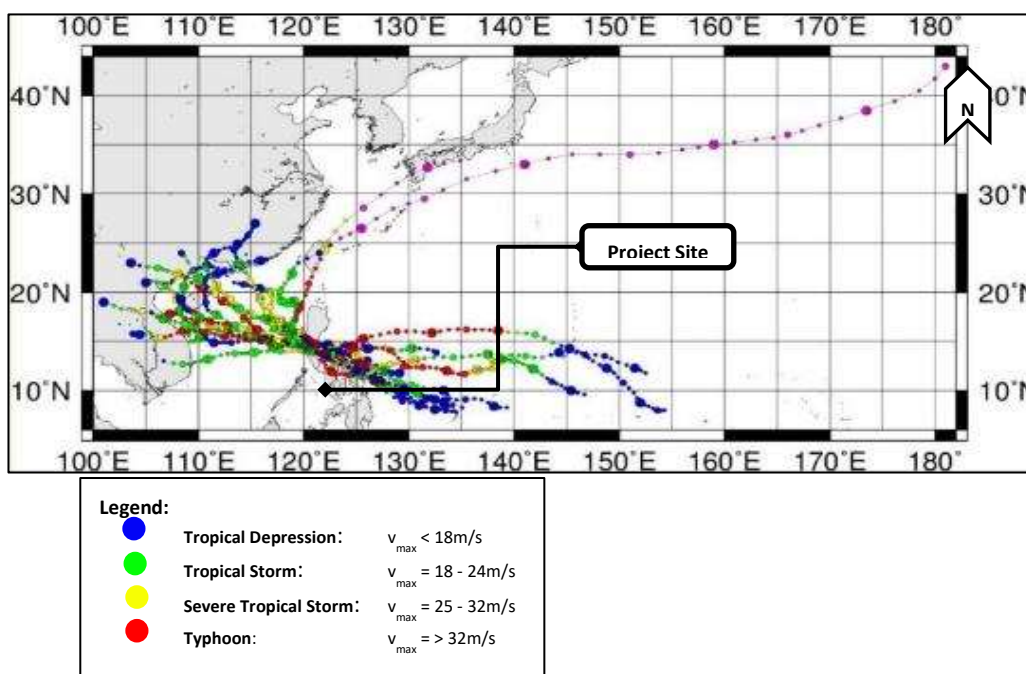
Figure 2.2-45 Typhoon Tracks within 200km of Project Site
