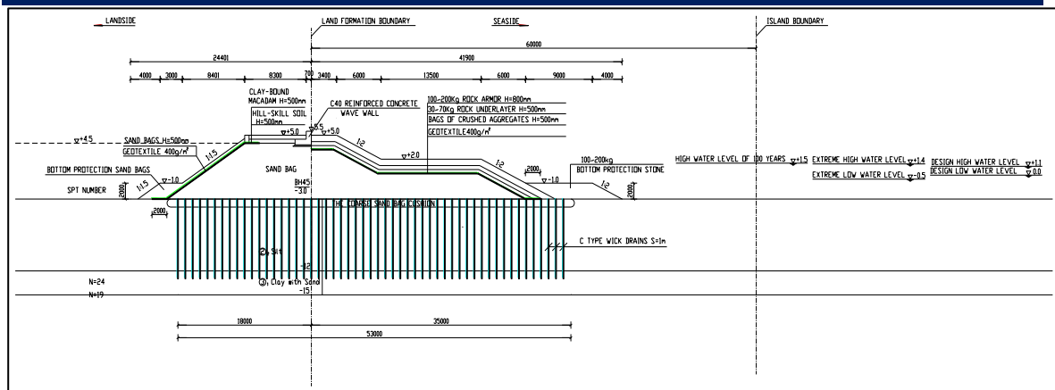
Plate 1-12 Sand bag dike + rock armor + wick drains
