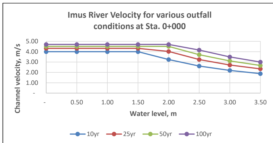
Figure 2.2-30 Imus River Profile at Various Outfall Conditions (100-year Return Period)
