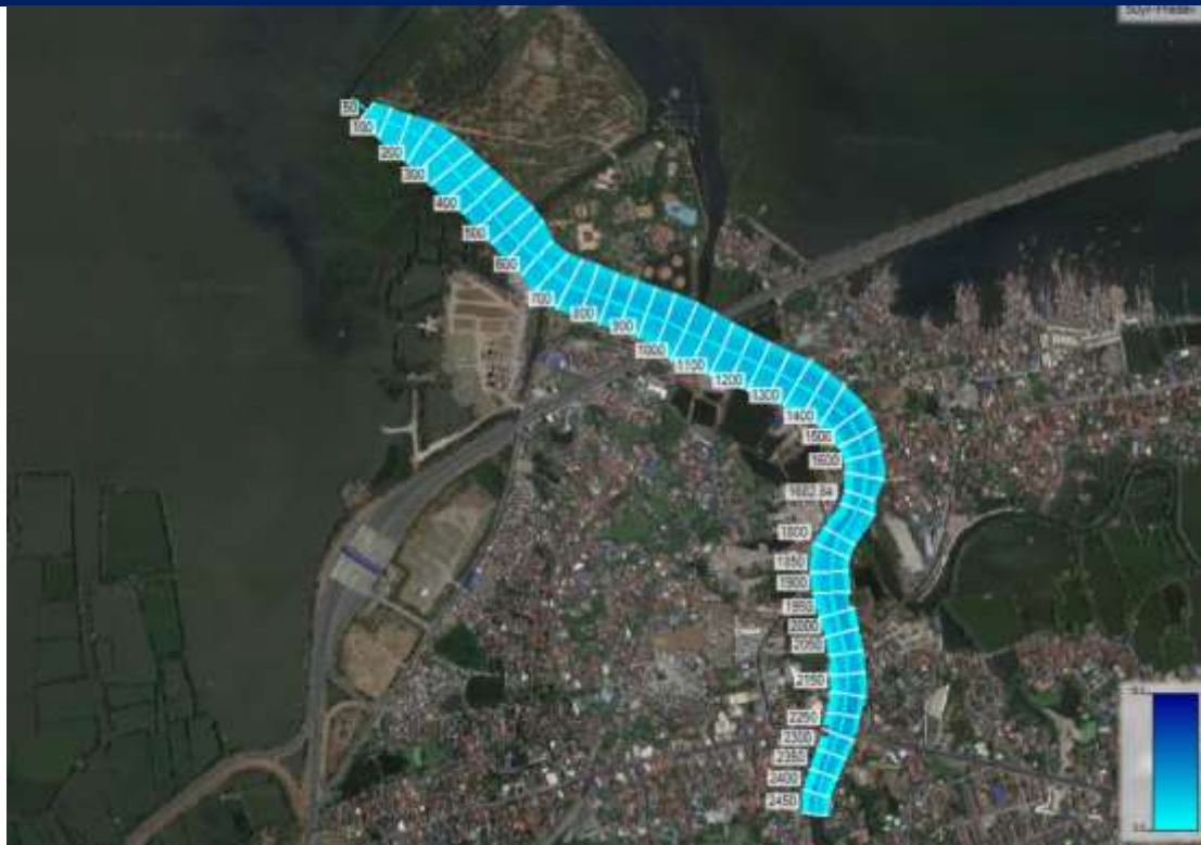
Figure 2.2-23 Inundation map of Imus River for 50-yr Return Period (Pre-development and Post-development Condition)
