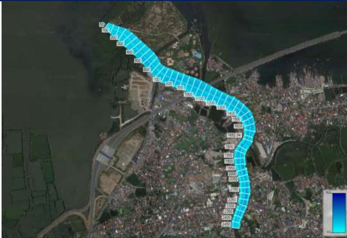
Figure 2.2-19 Inundation map of Imus River for 100-yr Return Period (based on highest historical water level at Manila South Tide Station)
