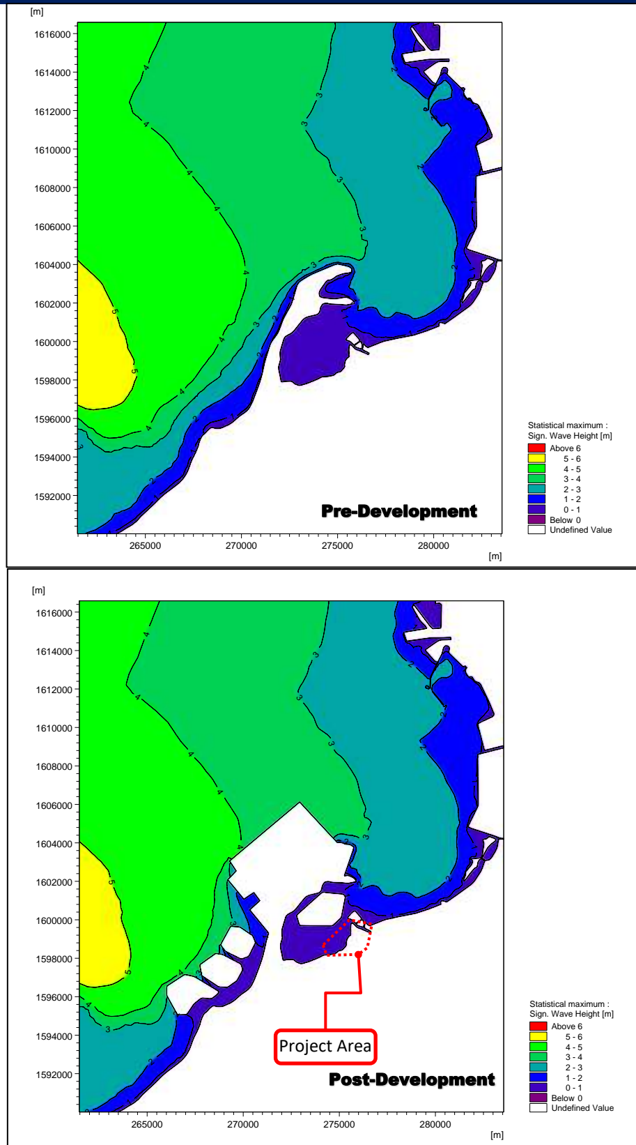
Figure 2.2-88 Simulated Max Significant Wave Heights for Typh. Xangsane/Milenyo (2006) Pre- & Post Development
