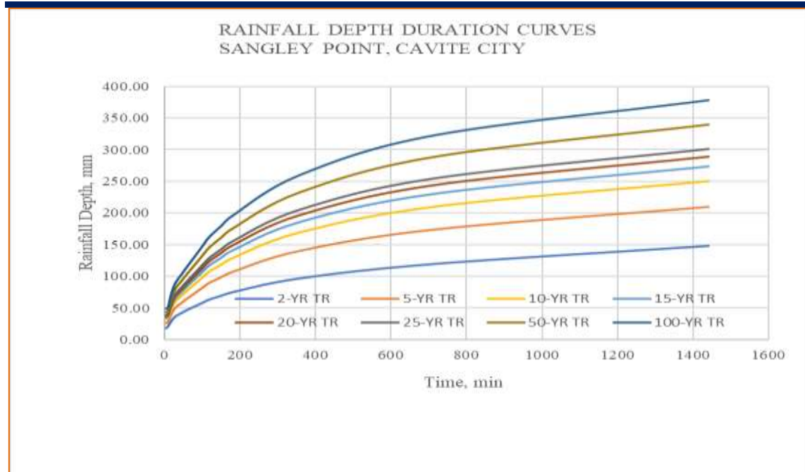
Figure 2.2-42 Rainfall Depth Duration Curves, Sangley Point, Cavite City
