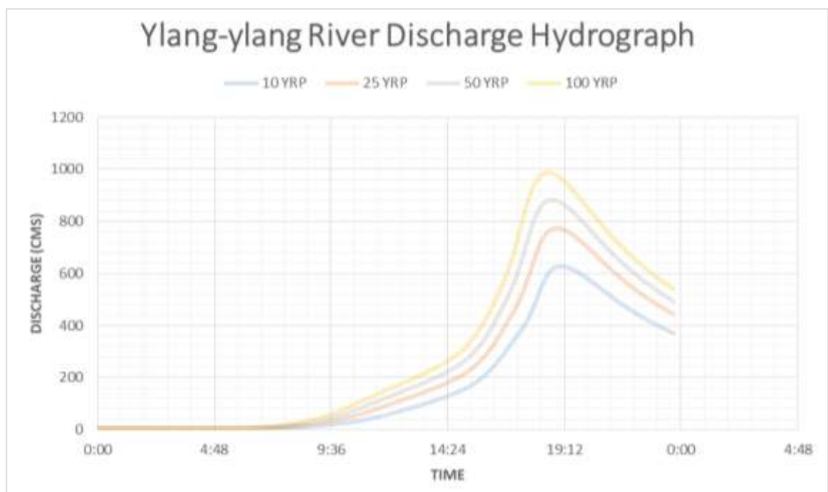
Figure 2.2-13 Ylang-ylang River Discharge Hydrograph
