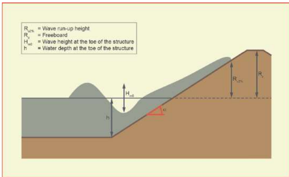
Figure 2.2-89 Wave Runup on a Smooth Impermeable Slope
