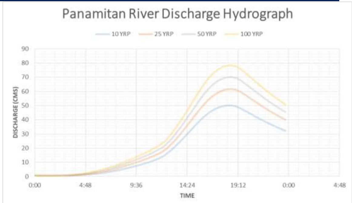
Figure 2.2-14 Panamitan River Discharge Hydrograph
