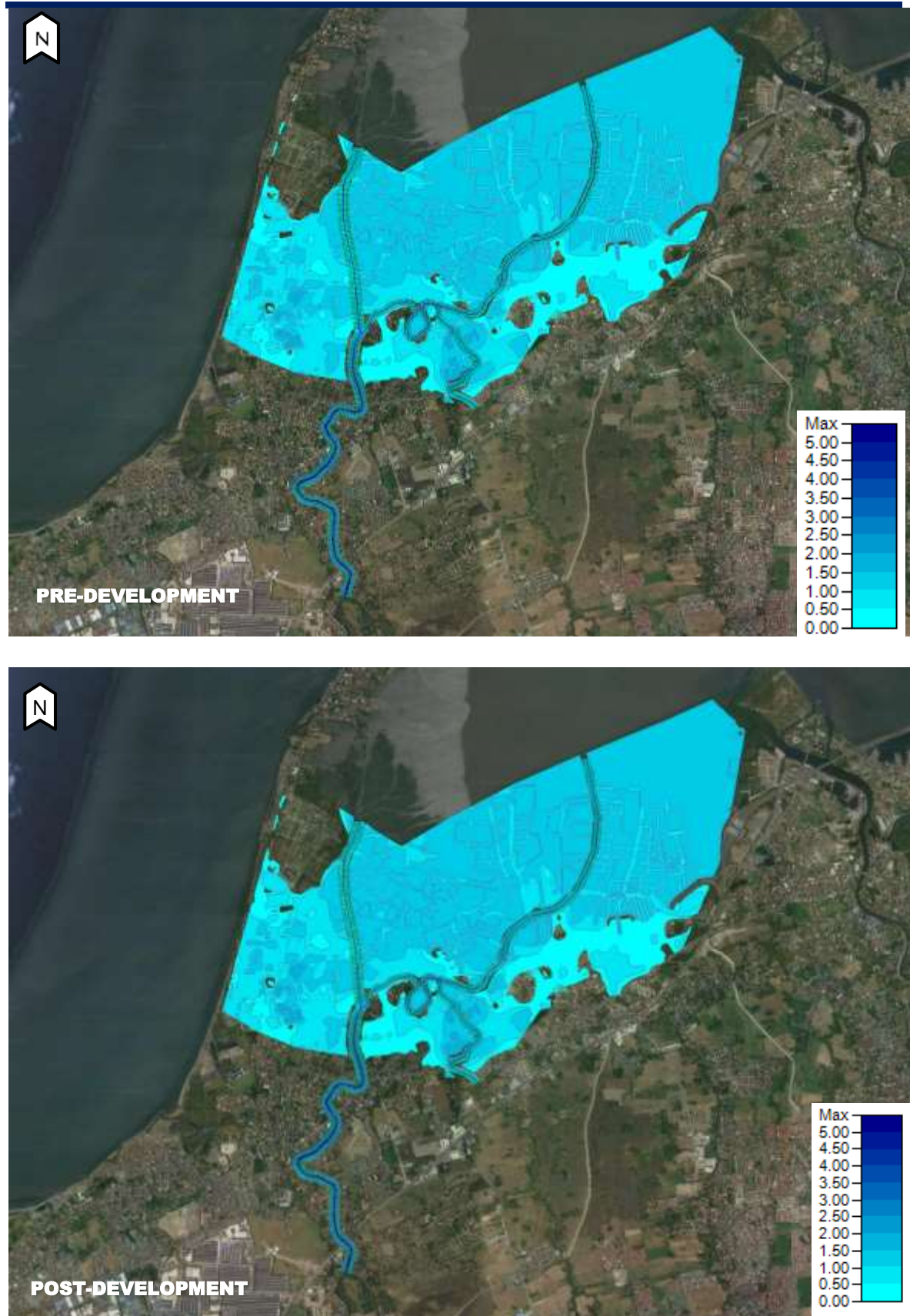
Figure 2.2-34 Flood Inundation Maps - 10-year Return Period
