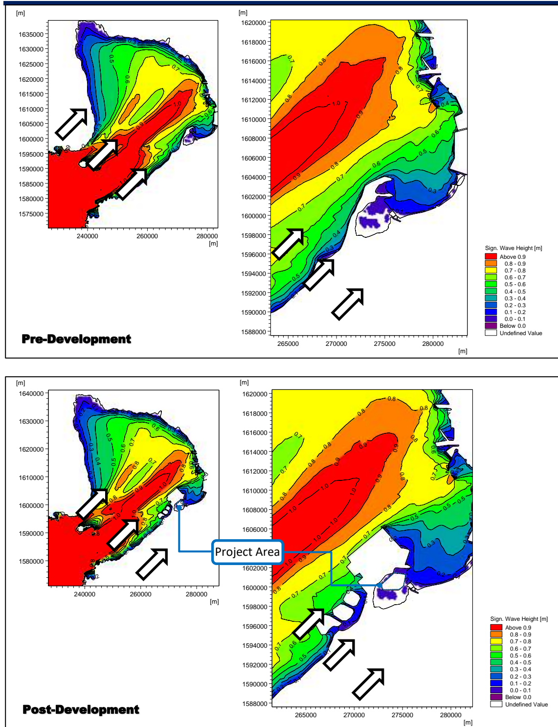
Figure 2.2-65 Wave Climate due to 5-8 mps Surface Winds & Offshore Waves from SW at MHHW (Pre- & Post-Dev't)
