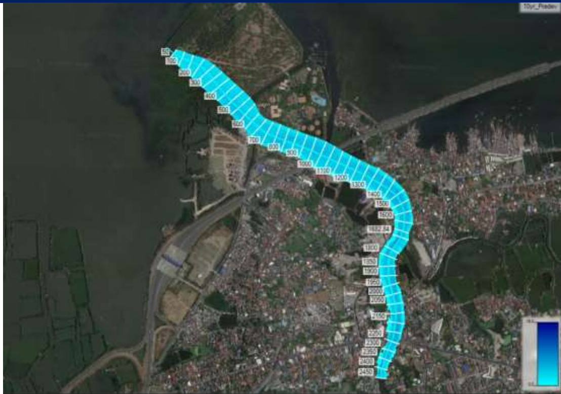
Figure 2.2-21 Inundation map of Imus River for 10-yr Return Period (Pre-development and Post-development Condition)
