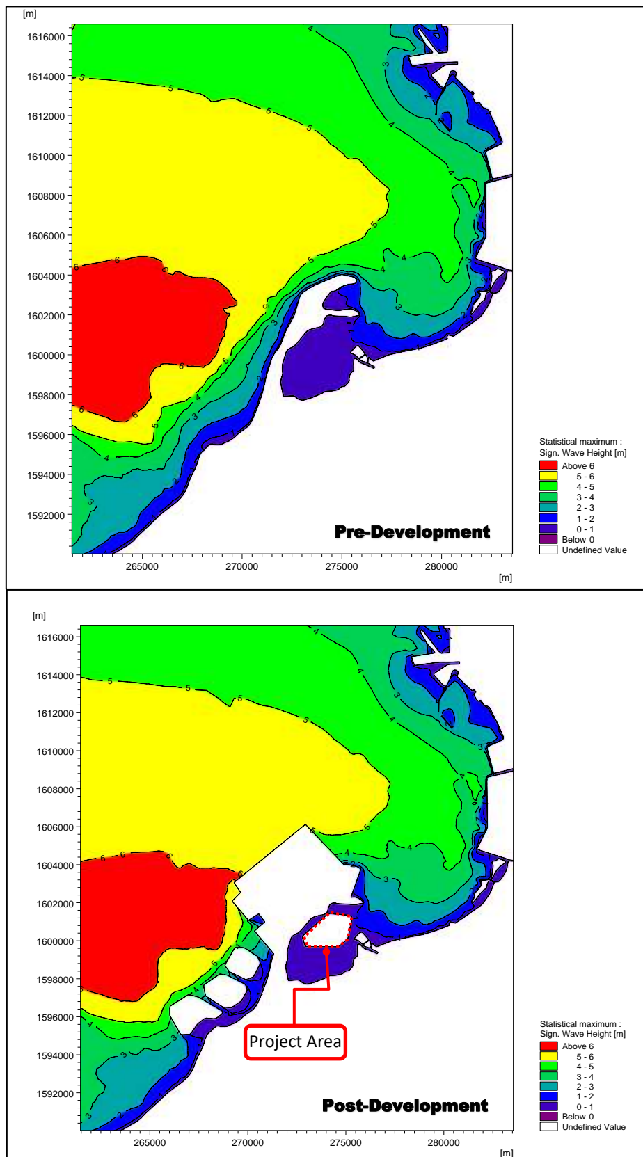
Figure 2.2-87 Simulated Max Significant Wave Heights for Typh. Patsy/Yoling (1970) Pre- & Post Development
