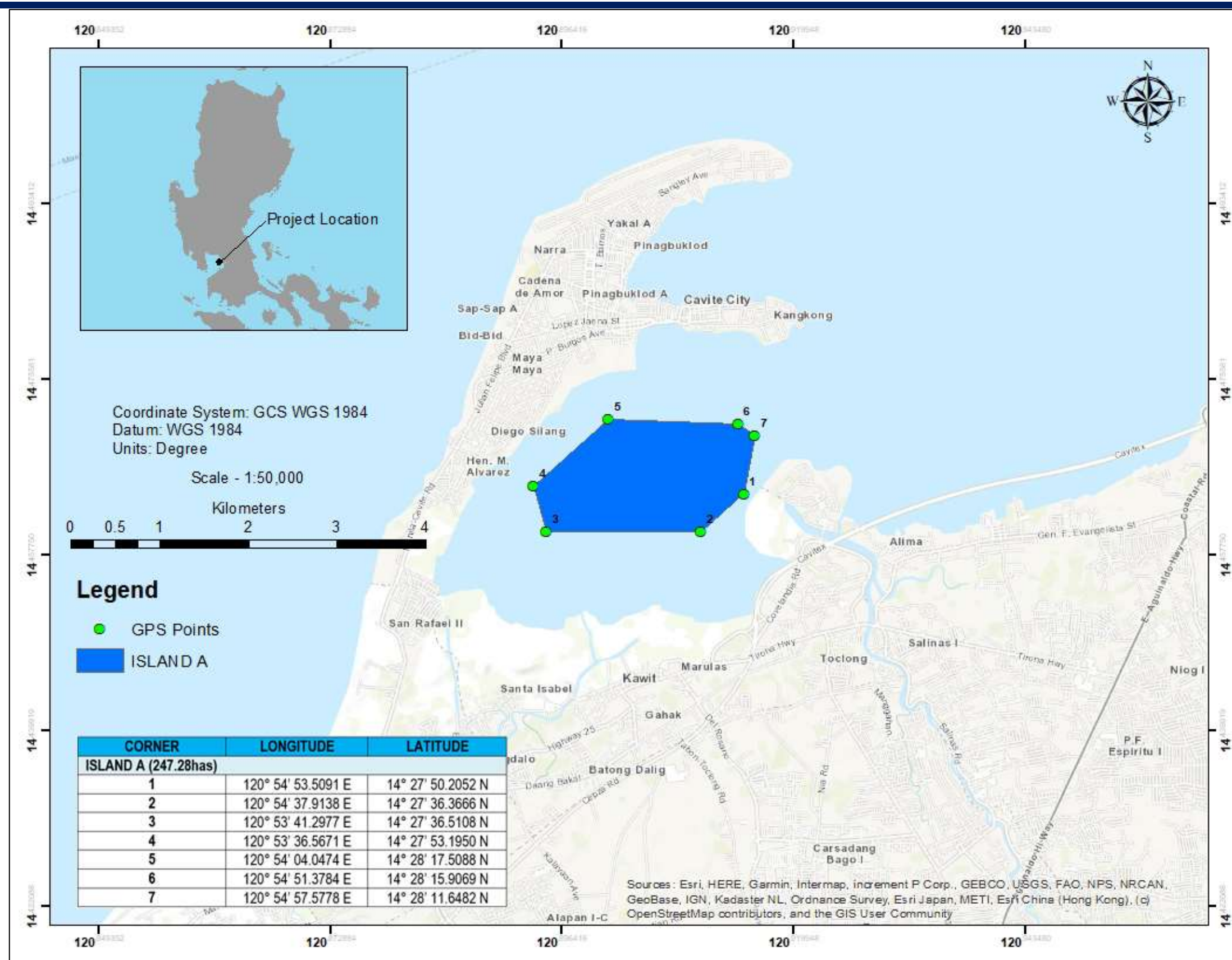
Figure 1-1. Project Site Location with Geographical Coordinate Points (NAMRIA Map)
