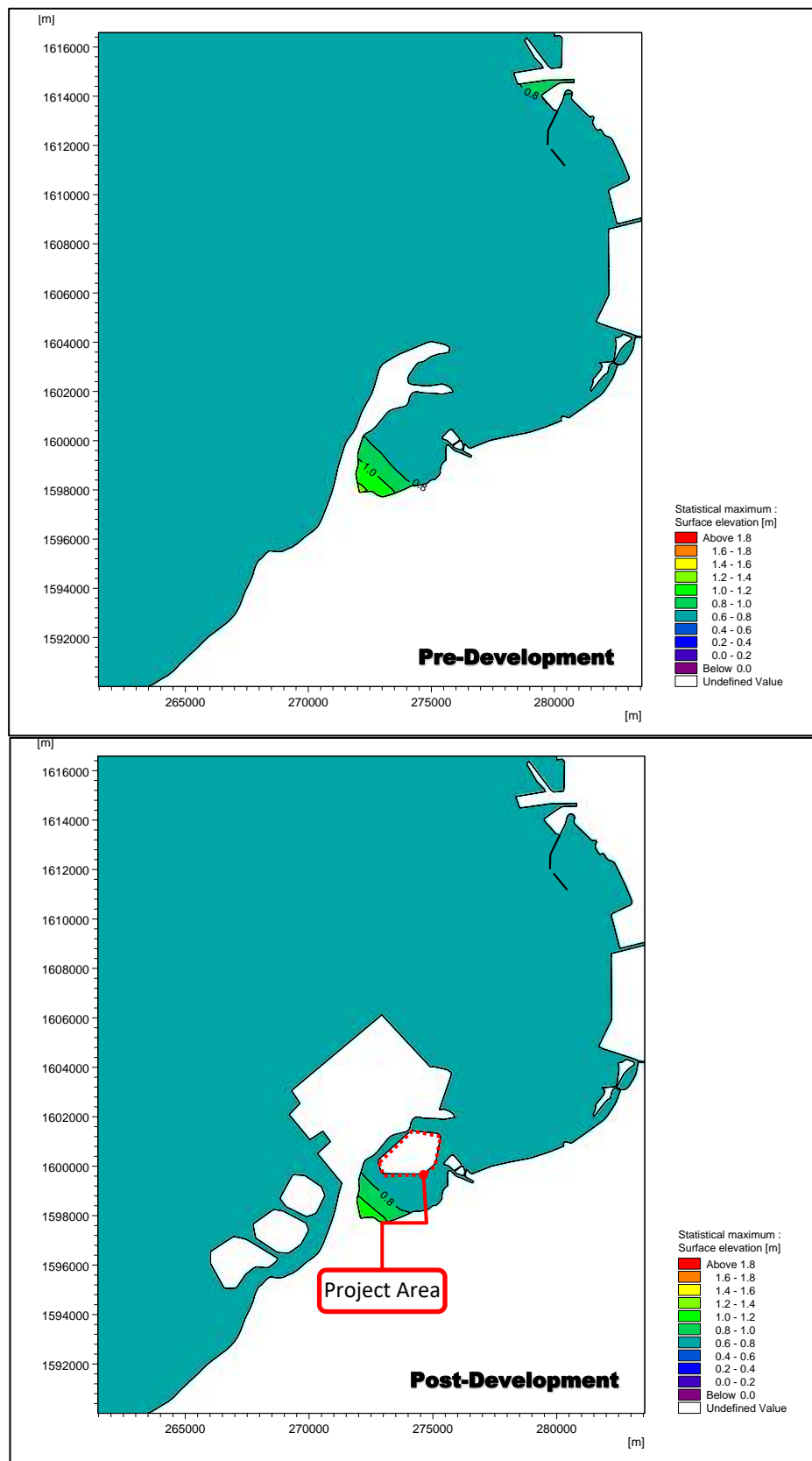
Figure 2.2-85 Simulated Storm Tide Level for Typhoon Xangsane/Milenyo (2006) Pre- & Post Development
