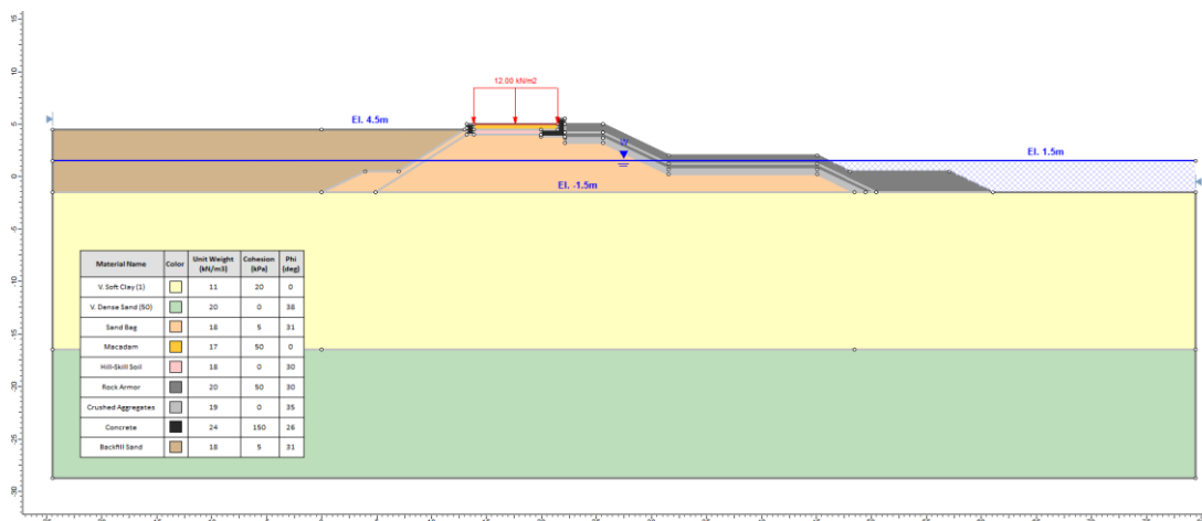
Figure 2.1-37 Slope Model of Island A Dike
