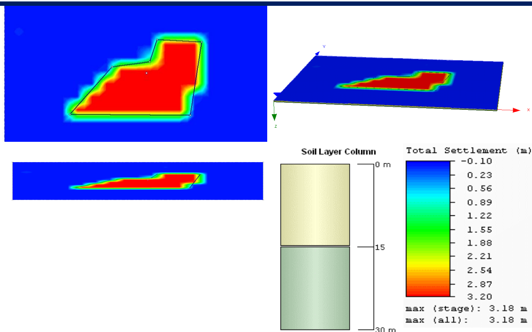
Figure 2.1-46 Settlement Analysis Results for 7m fill height
