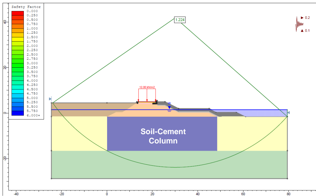
Figure 2.1-41 Case 2: Earthquake (FoS=1.224)
