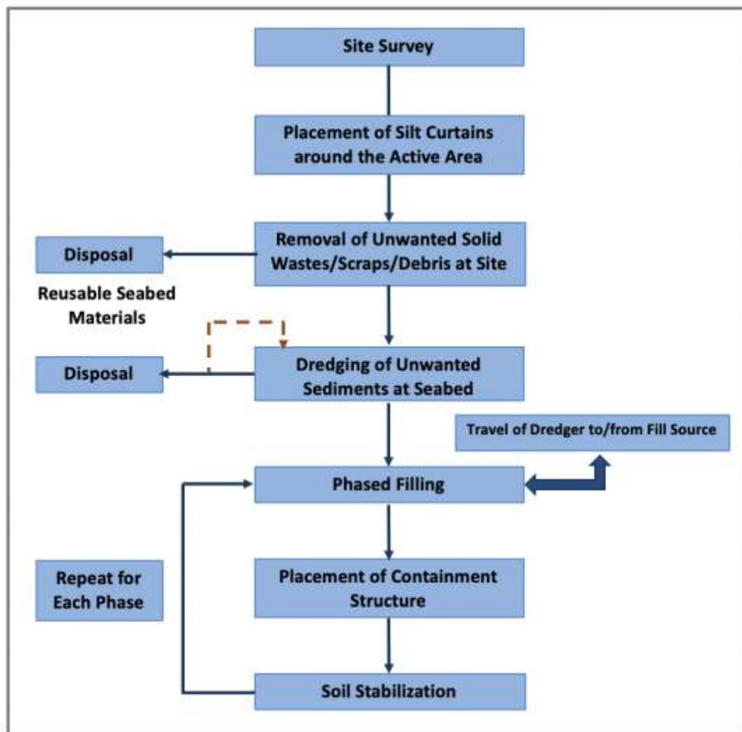
Figure 1-11 Process Flow Diagram for Reclamation Projects
