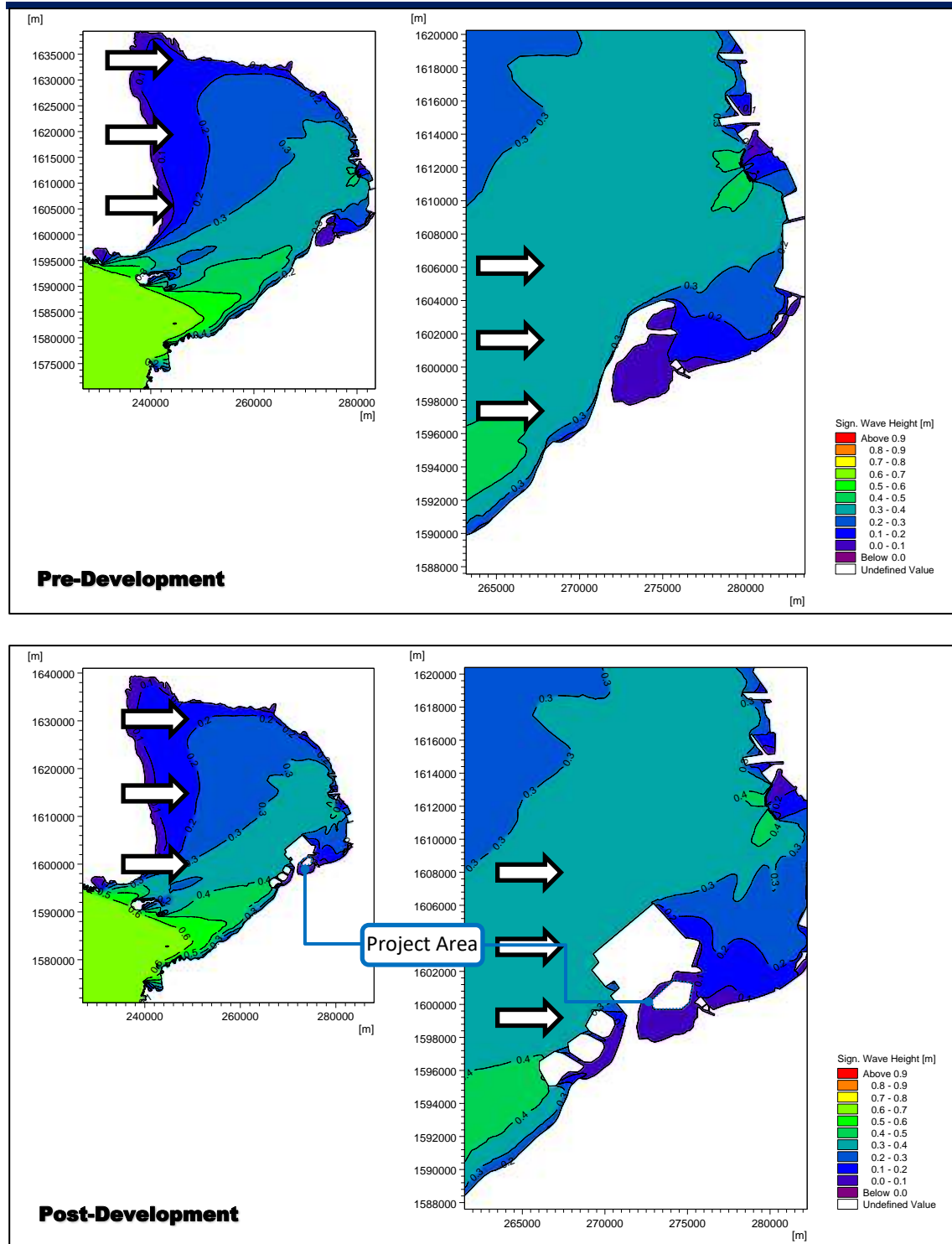
Figure 2.2-70 Wave Climate due to 1-4 mps Surface Winds & Offshore Waves from W at MHHW (Pre- & Post-Dev't)
