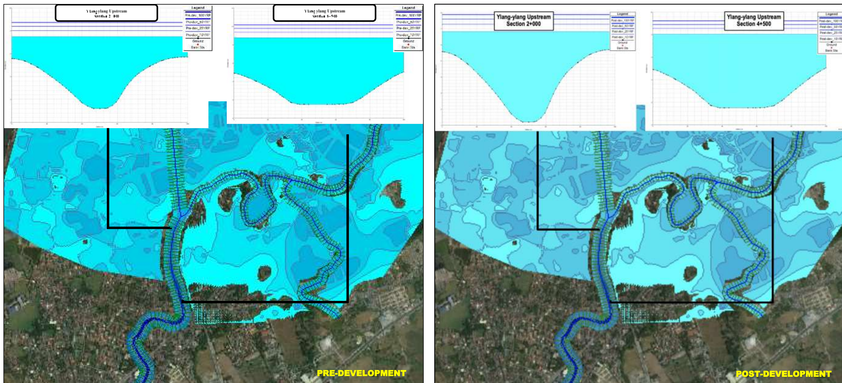
Figure 2.2-39 Ylang-ylang River Upstream Sections (Sta 2+000 & Sta 4+500)
