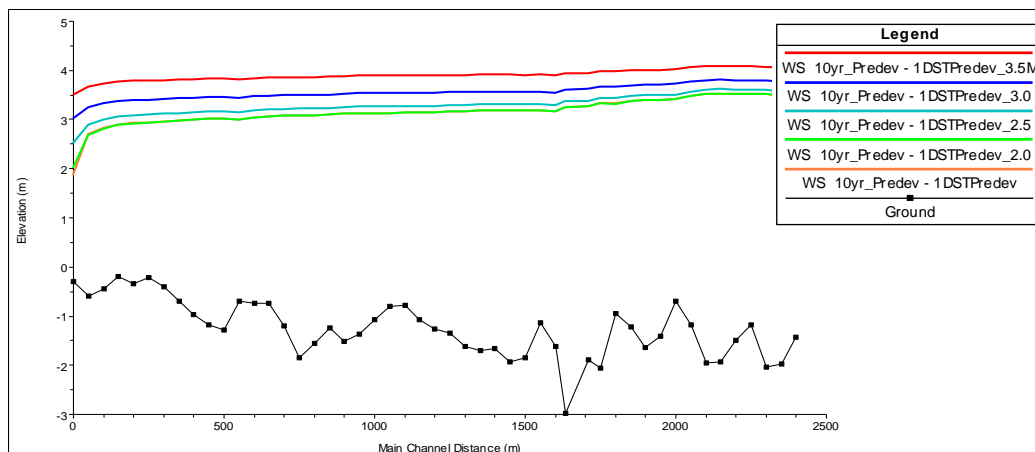
Figure 2.2-27 Imus River Profile at various outfall conditions (25-year Return Period)
