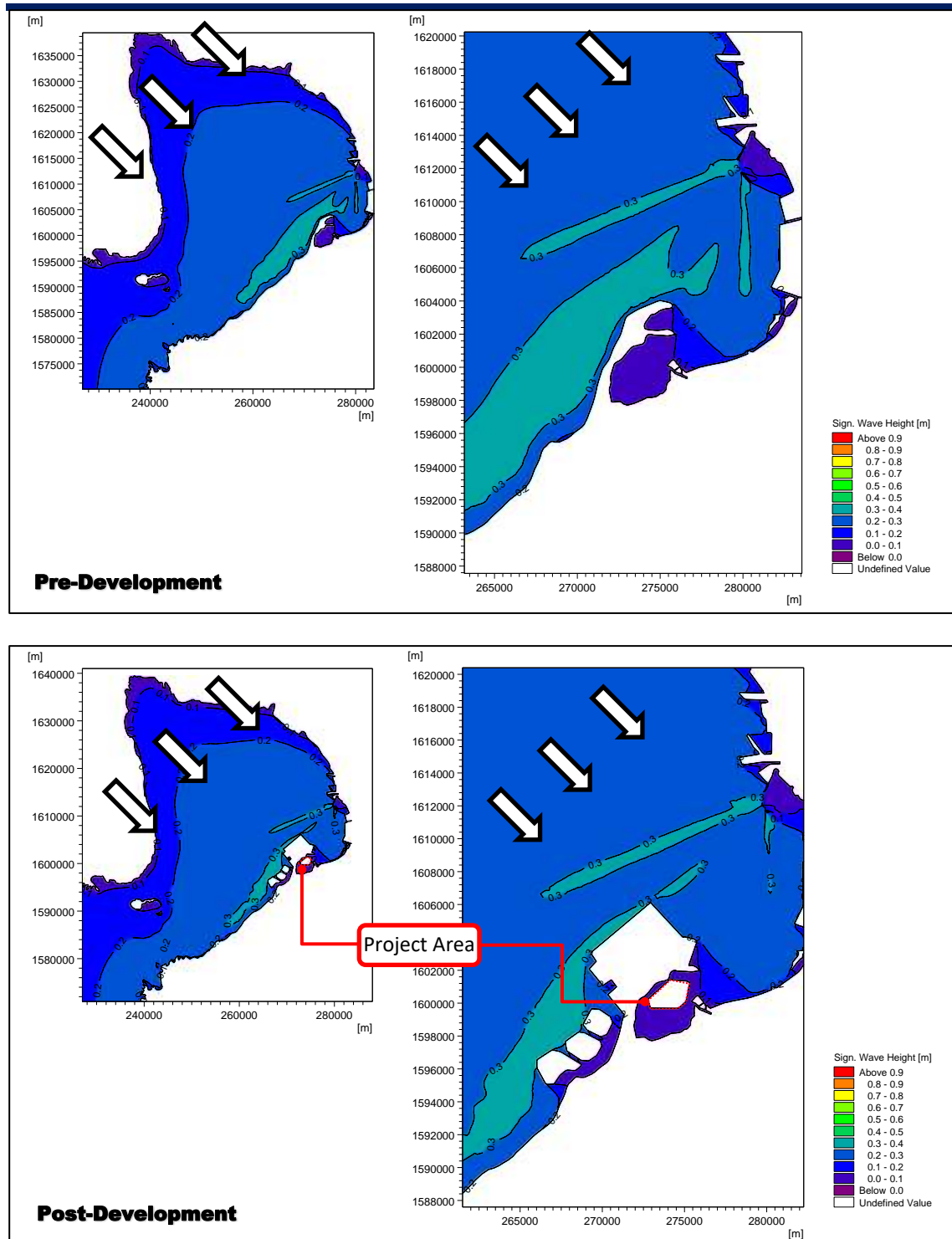
Figure 2.2-72 Wave Climate due to 1-4 mps Surface Winds & Offshore Waves from NW at MHHW (Pre- & Post-Dev't)
