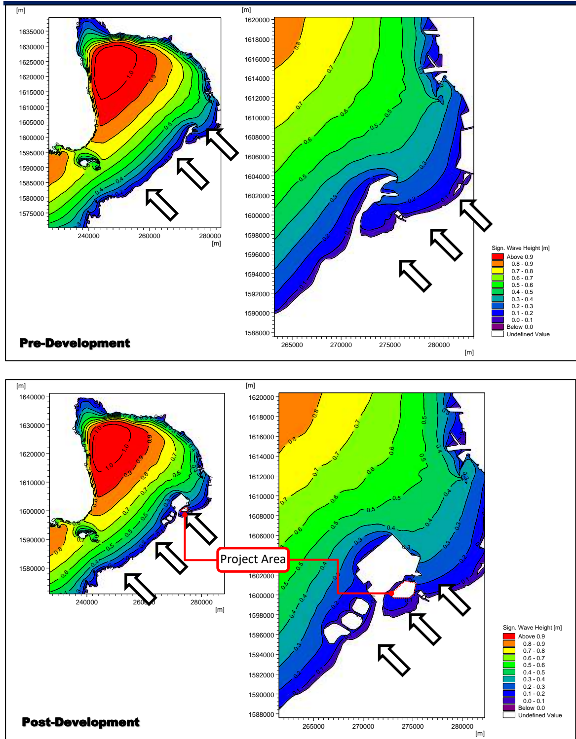
Figure 2.2-63 Wave Climate due to 5-8 mps Surface Winds & Offshore Waves from SE at MHHW (Pre- & Post-Dev't)
