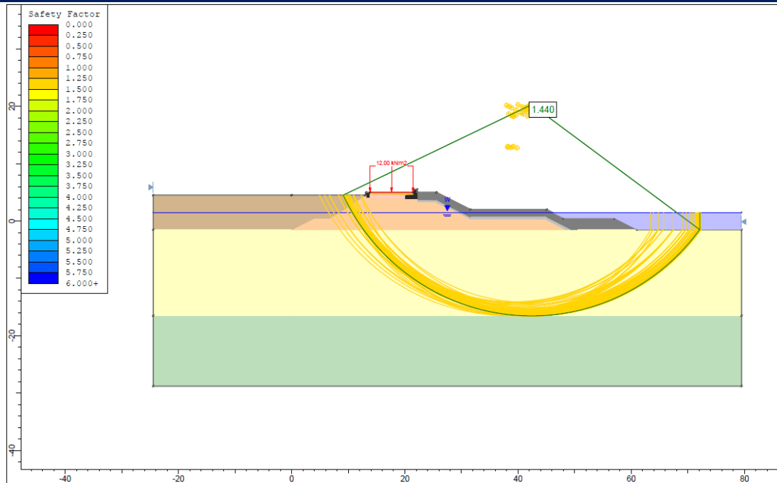
Figure 2.1-38 Case 1: Static (FoS=1.440)
