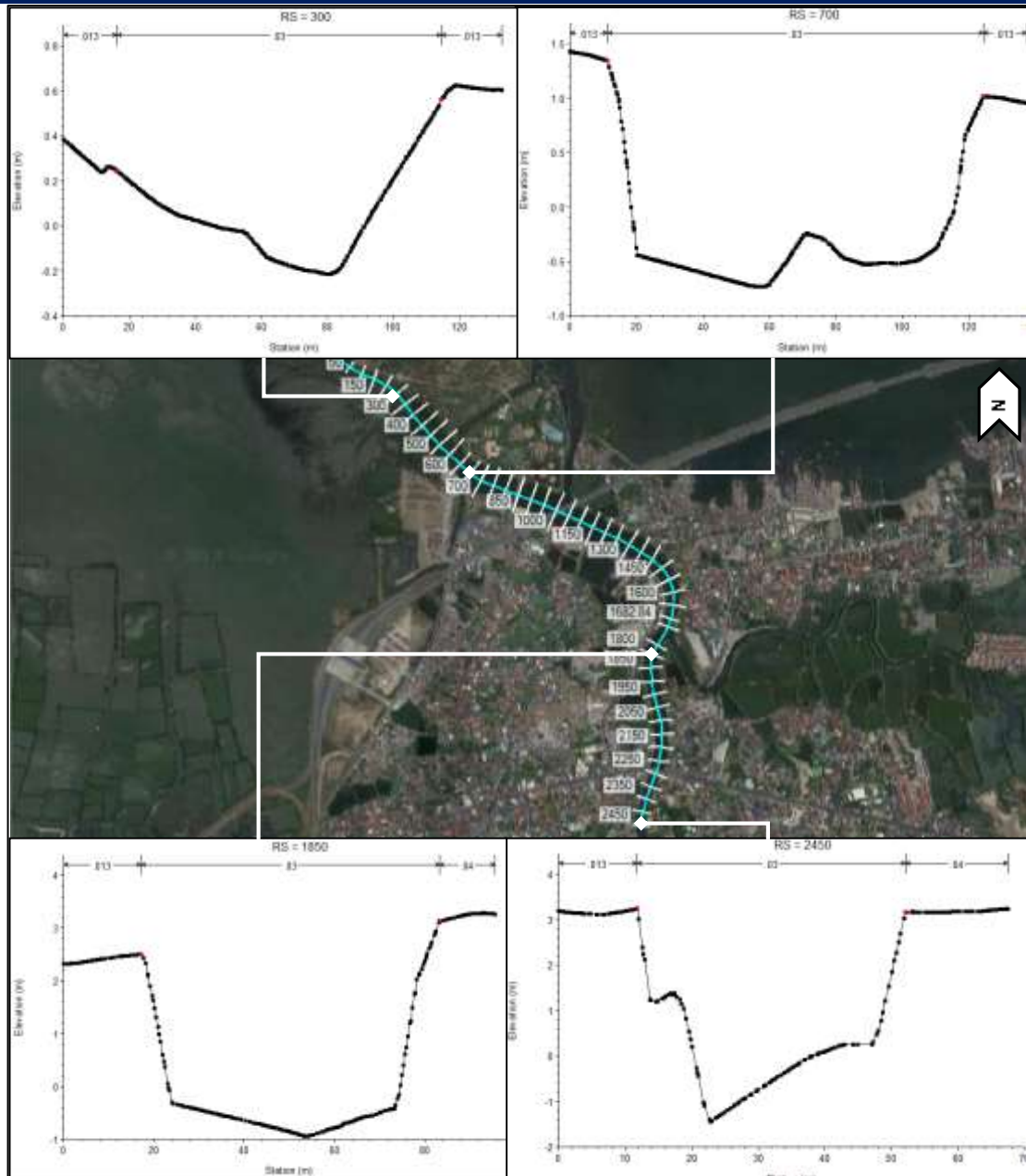
Figure 2.2-15 HEC-RAS Model and Sample Sections for Imus River
