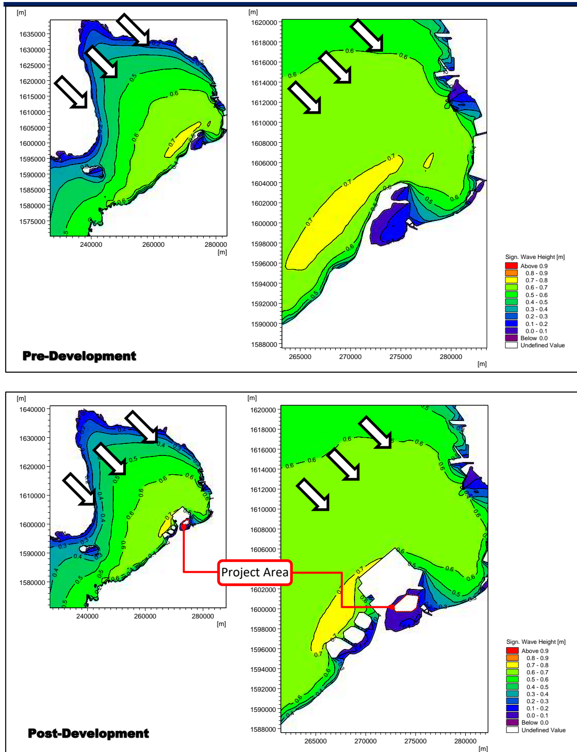
Figure 2.2-73 Wave Climate due to 5-8 mps Surface Winds & Offshore Waves from NW at MHHW (Pre- & Post-Dev't)
