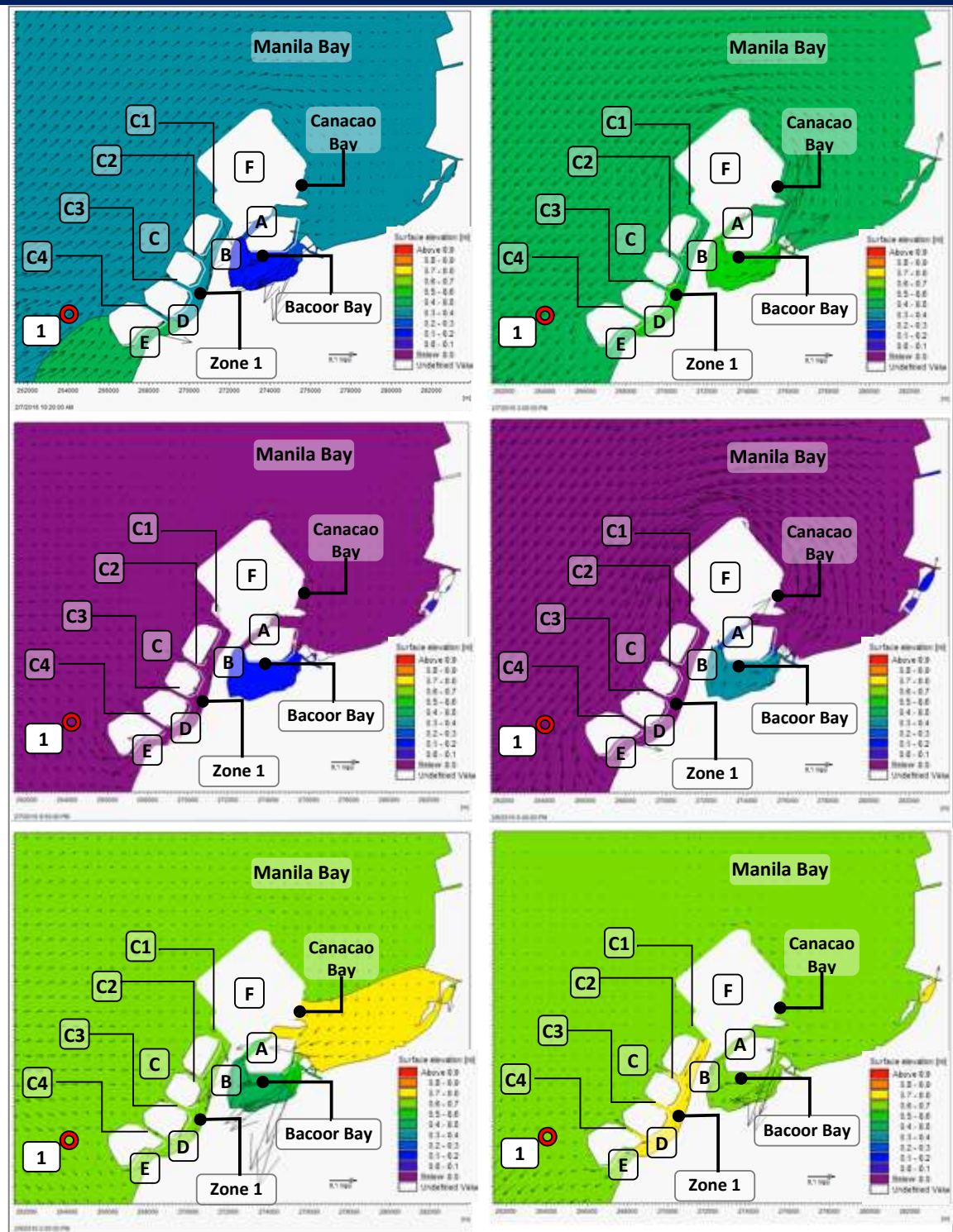
Figure 2.2-78 Chronological Snapshots of Tidal Currents During Jan. 29 – Feb 20, 2016
