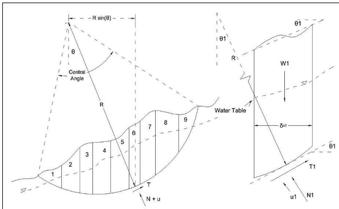
Figure 2.1-35 Stability analysis by Limit-Equilibrium Methods
