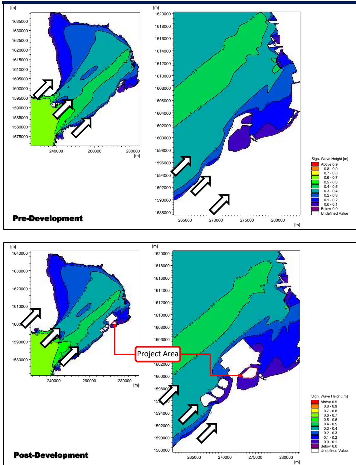
Figure 2.2-64 Wave Climate due to 1-4 mps Surface Winds & Offshore Waves from SW at MHHW (Pre- & Post-Dev't)
