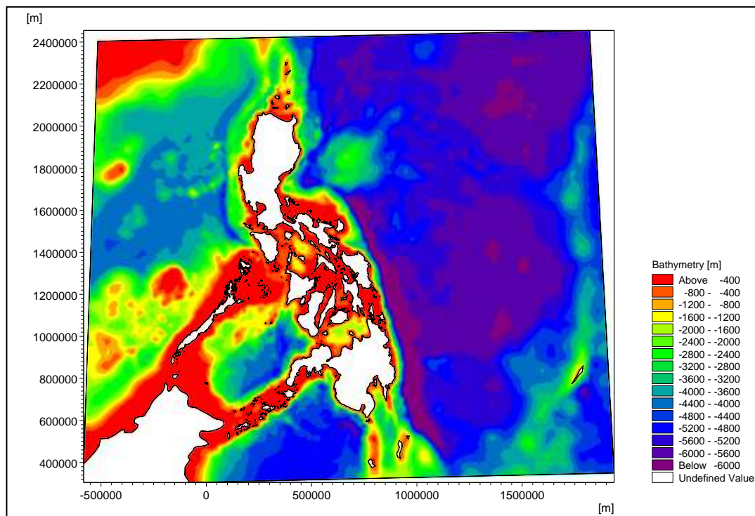
Figure 2.2-51 Domain extents for the hydrodynamic computation of the regional model
