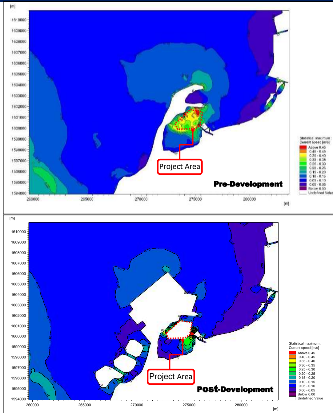
Figure 2.2-77 Maximum current (Jan. 29, 2016 – Feb. 29, 2016) (Pre- & Post-Development)
