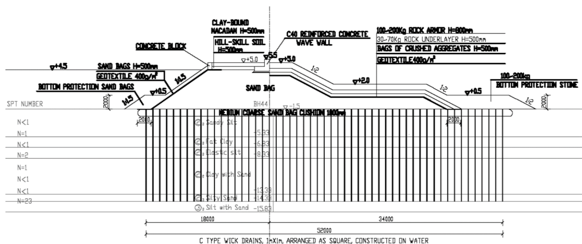
Figure 2.1-36 Section of Island A Dike (I)
