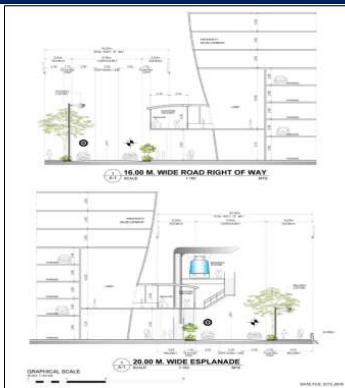
Figure 1-17. (Top Image) Suggested Section for the 16.0 m Wide RROW (Local Road) and Suggested Section for the 20.0 m Wide RROW (Esplanade) for the Proposed Cavite (CAV) Island A Reclamation Project (247.28 has. GRSA)
