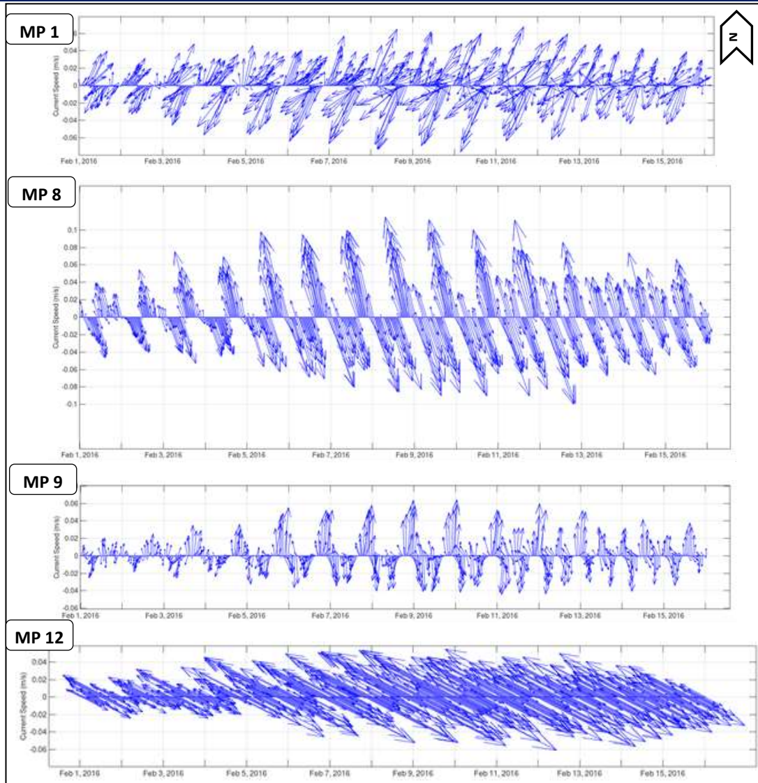
Figure 2.2-80 Tidal Current Time Histories Over 15 days at Monitoring Points 1, 8, 9 & 12
