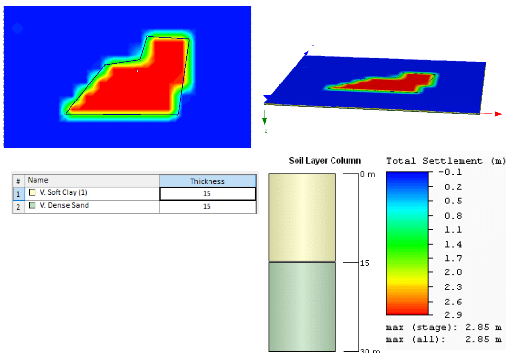
Figure 2.1-45 Settlement Analysis Results for 5m fill height
