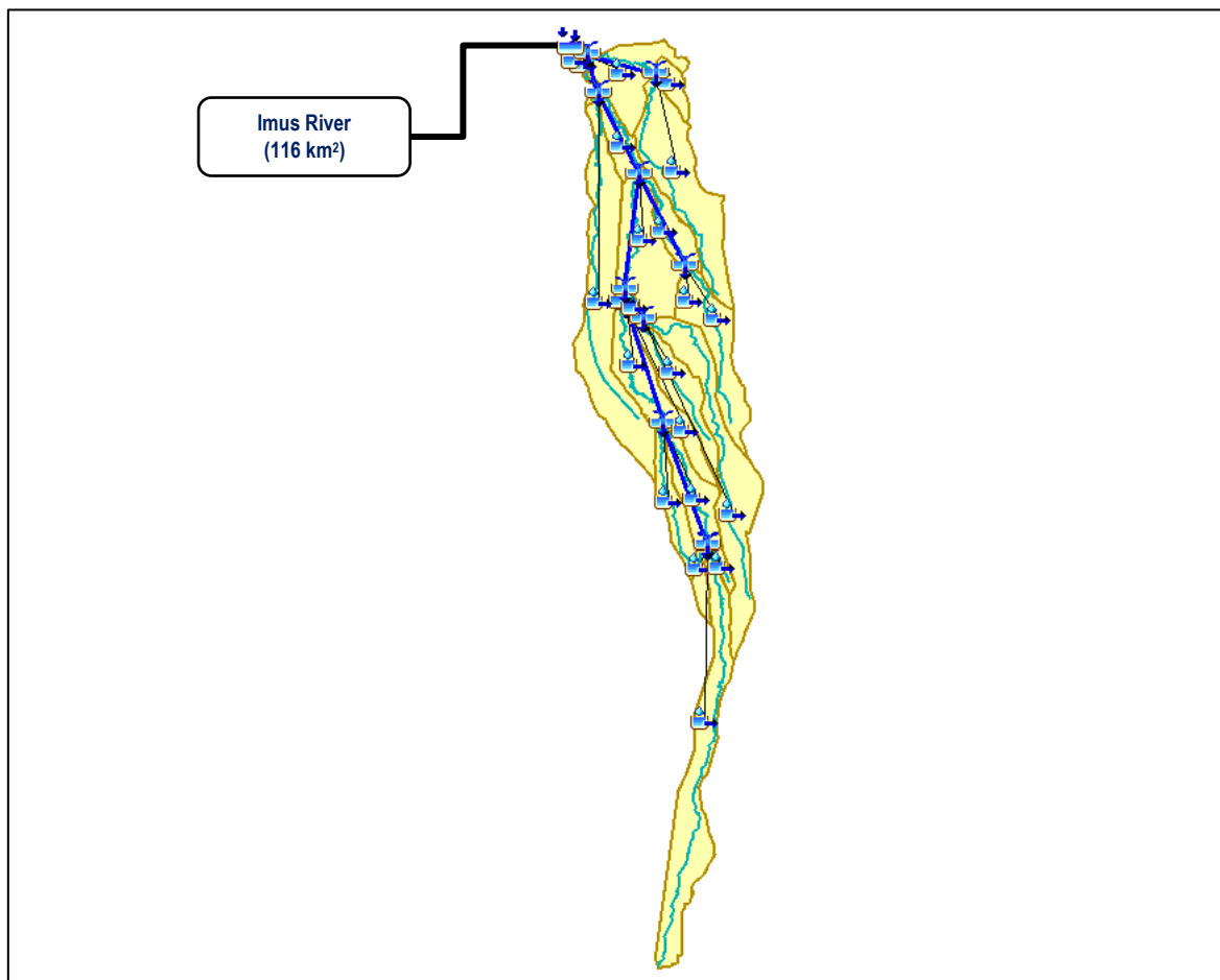
Figure 2.2-10 HEC-HMS Model for Imus River Catchment
