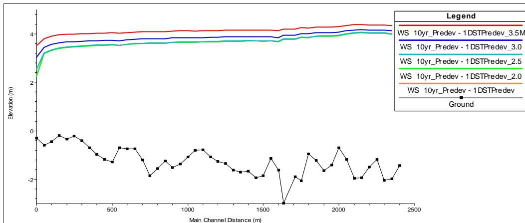
Figure 2.2-29 Imus River Profile at Various Outfall Conditions (100-year Return Period)
