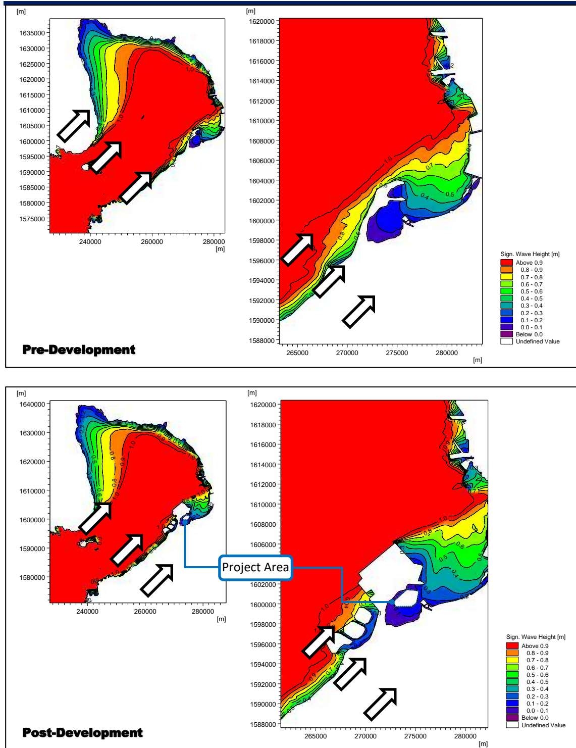
Figure 2.2-66 Wave Climate due to 9-12 mps Surface Winds & Offshore Waves from SW at MHHW (Pre- & Post-Dev't)
