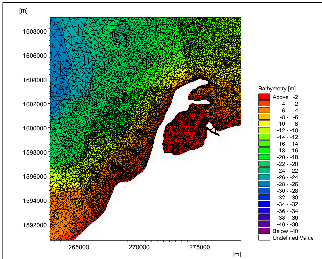
Figure 2.2-53 Local Model Mesh for the hydrodynamic computation at the site –(Pre-Dev)
