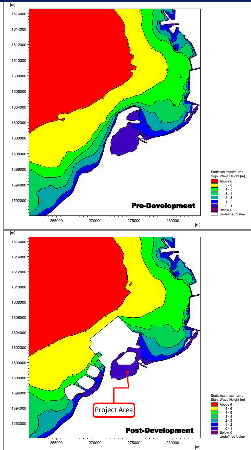
Figure 2.2-86 Simulated Max Significant Wave Heights for Typh. Rita/Kading (1978) Pre- & Post Development
