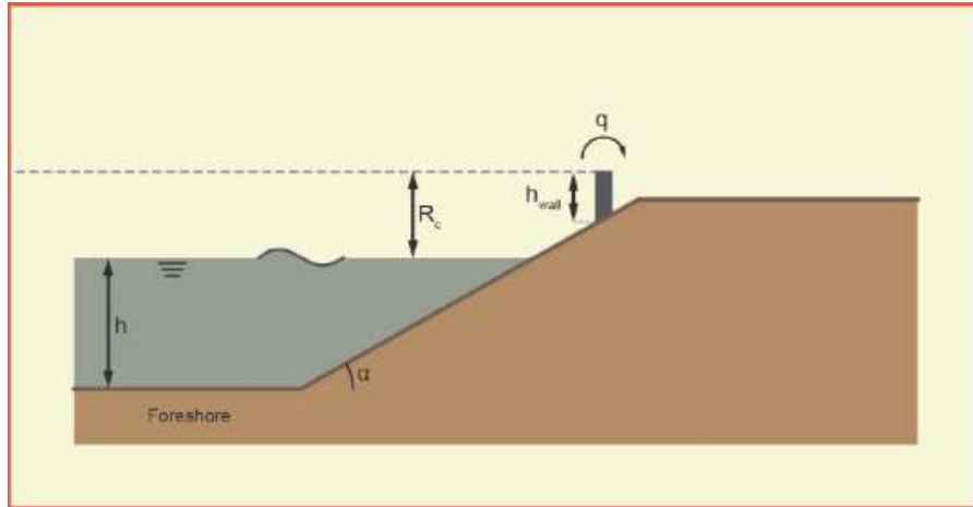
Figure 2.2-90 Overtopping Discharge of a Slope with Storm Wall
