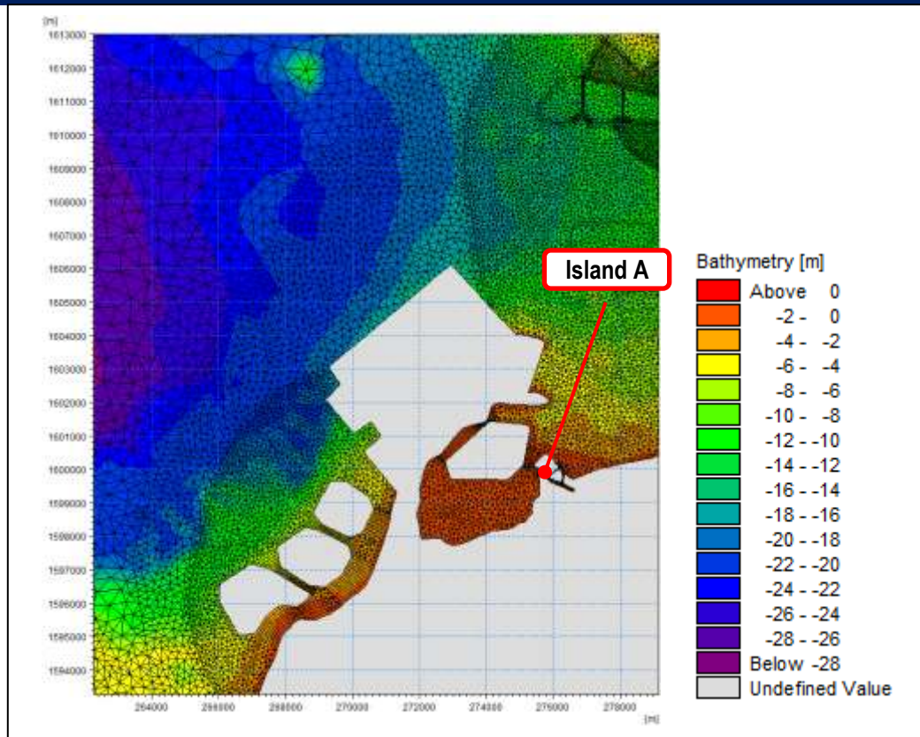
Figure 2.2-54 Local Model Mesh for the Hydrodynamic Computation at the Site (Post-Dev)
