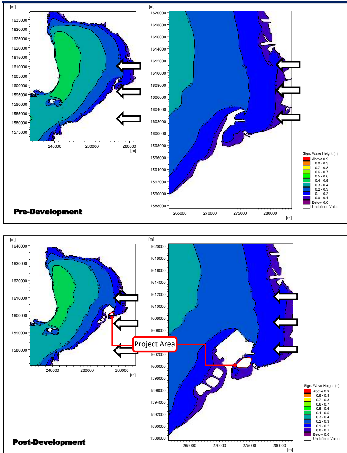
Figure 2.2-58 Wave Climate due to 1-4 mps Surface Winds & Offshore Waves from E at MHHW (Pre- & Post-Devt)
