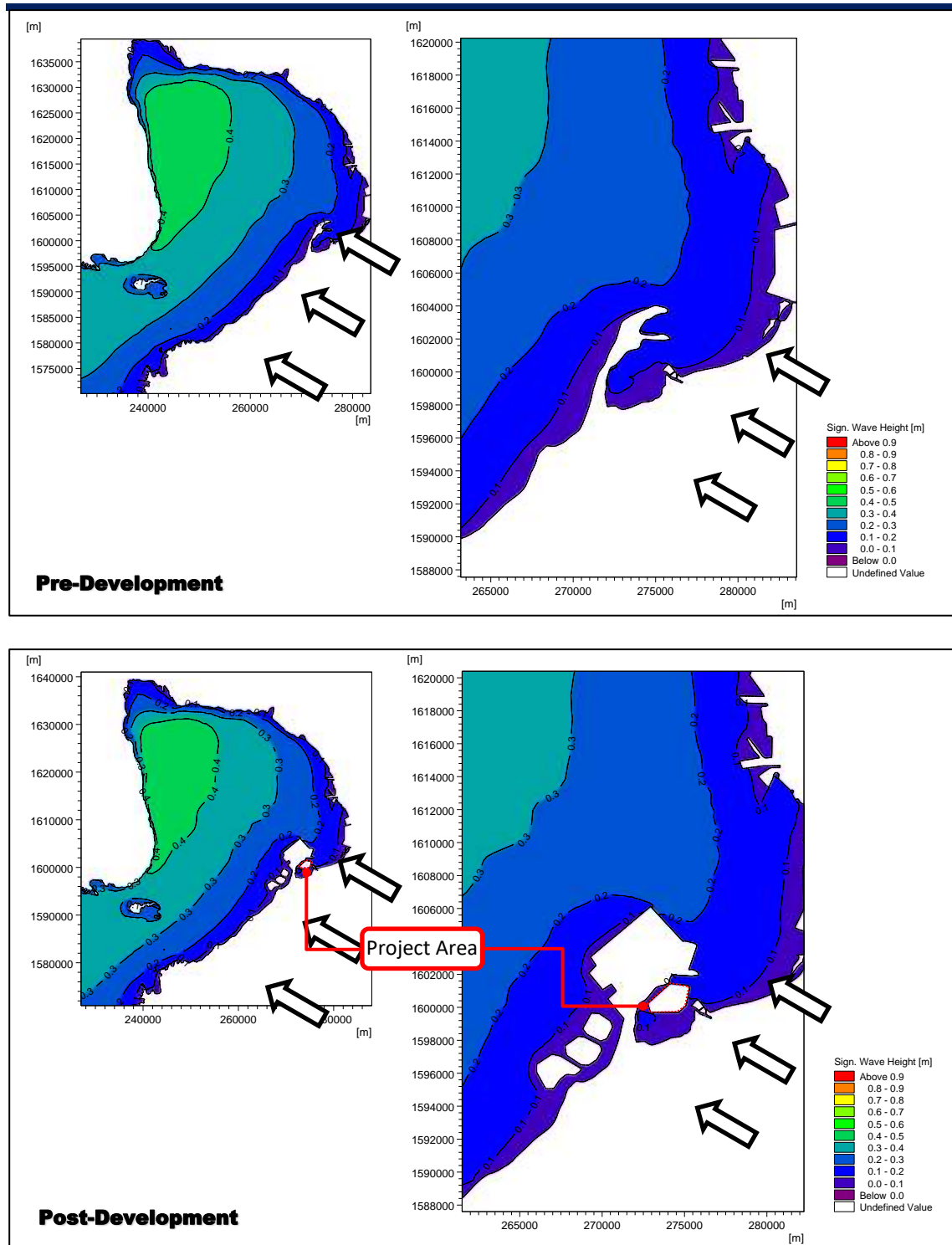
Figure 2.2-60 Wave Climate due to 1-4 mps Surface Winds & Offshore Waves from ESE at MHHW (Pre- & Post-Dev't)
