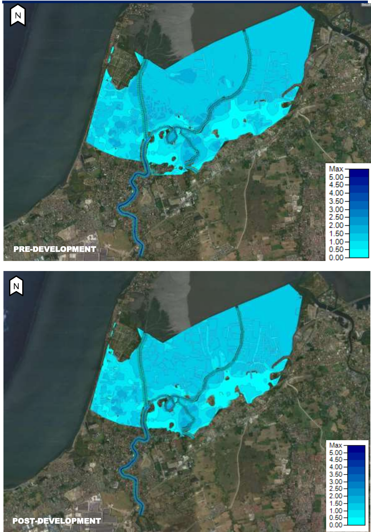
Figure 2.2-35 Flood Inundation - 25-year Return Period
