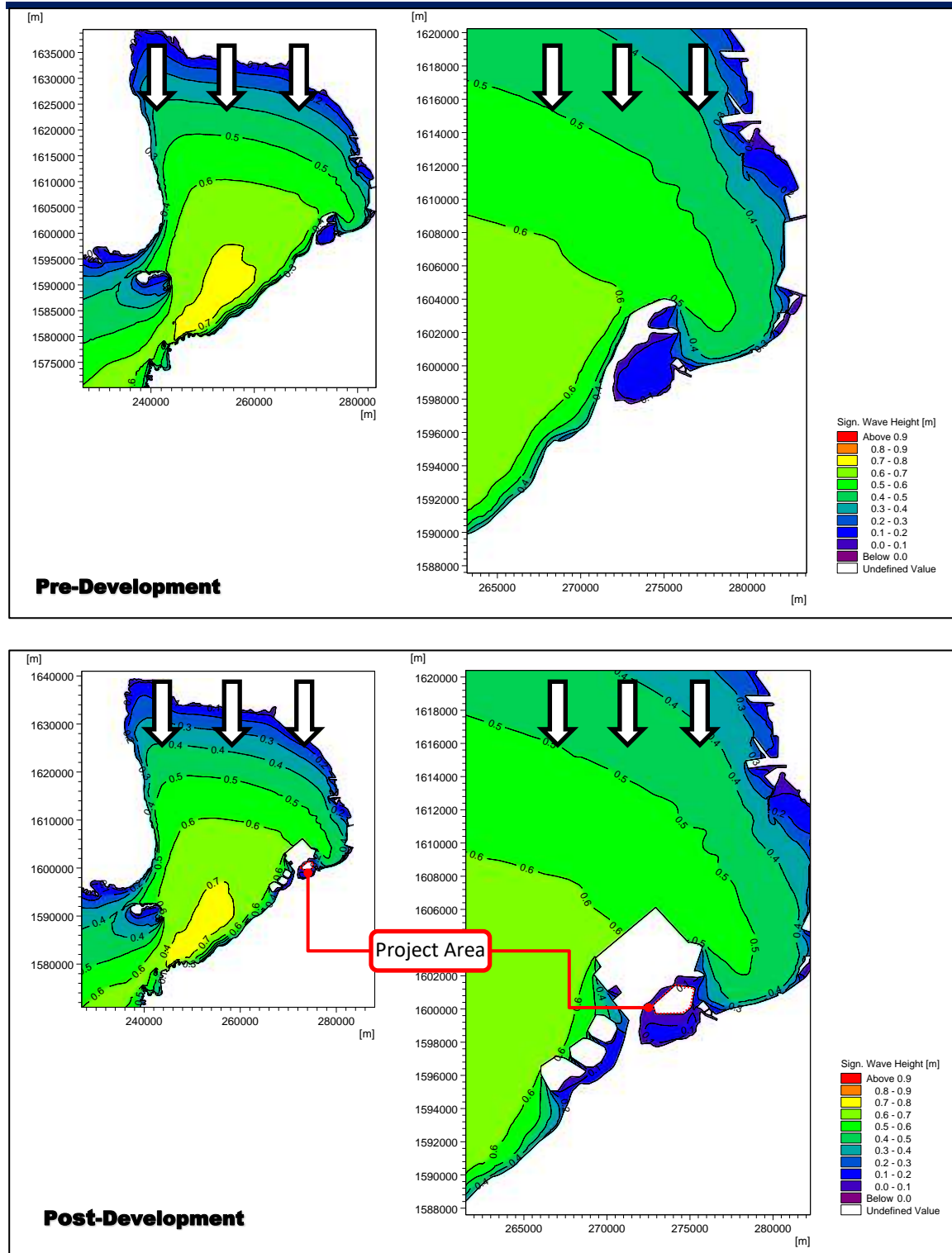
Figure 2.2-57 Wave Climate due to 5-8 mps Surface Winds & Offshore Waves from N at MHHW (Pre- & Post-Dev't)
