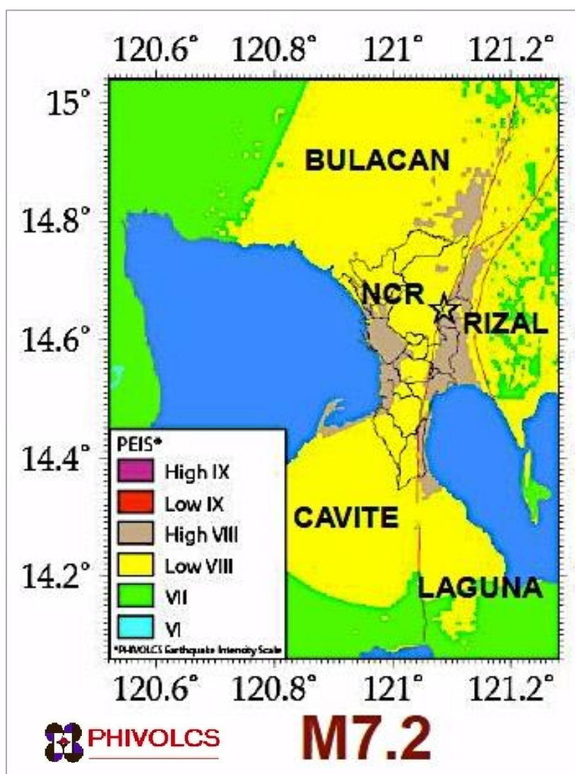
Figure 2.1-24 Ground Shaking in Greater Metro Manila and Vicinities (WVF Earthquake)
