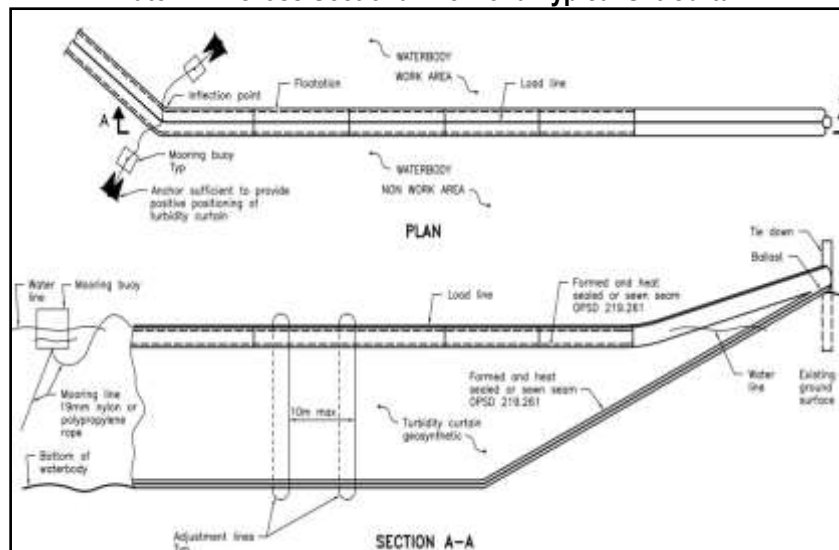
Plate 1-11. Cross Sectional View of a Typical Silt Curtain
