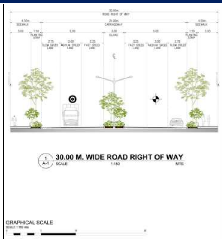
Figure 1-15. Suggested Section for the 30.0 m Wide RROW (Spine Road) for the Proposed Cavite (CAV) Island A Reclamation Project (247.28 has. GRSA)
