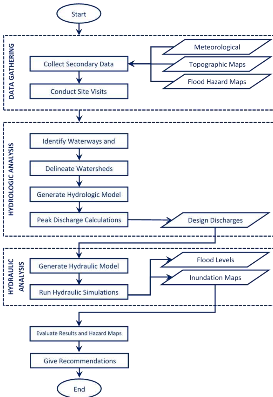
Plate 2.2-2. Flood Studies Process Flow Diagram
