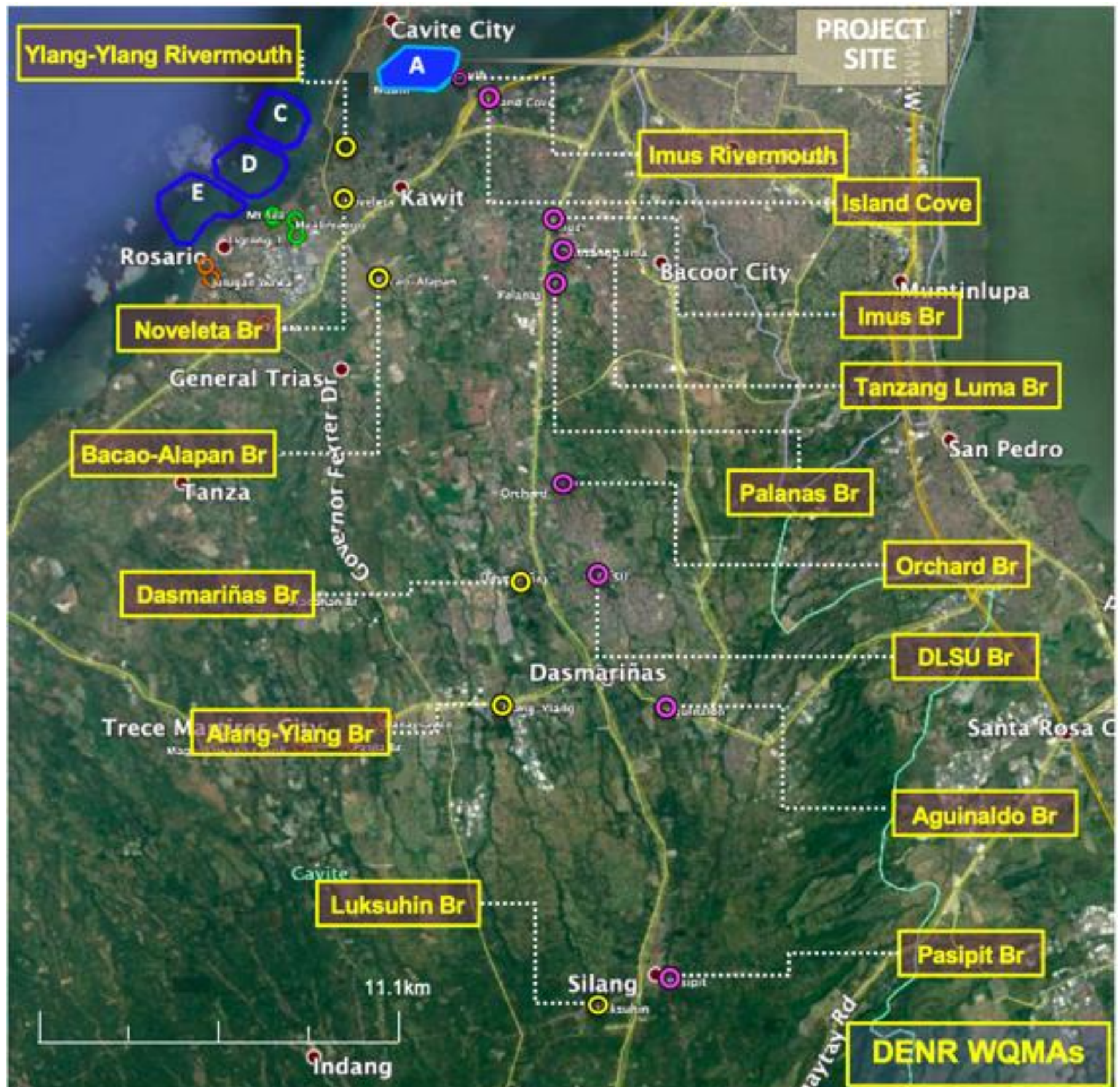
Figure 2.2-98 Location Map of Ylang-ylang and Imus Rivers WQMA Stations
