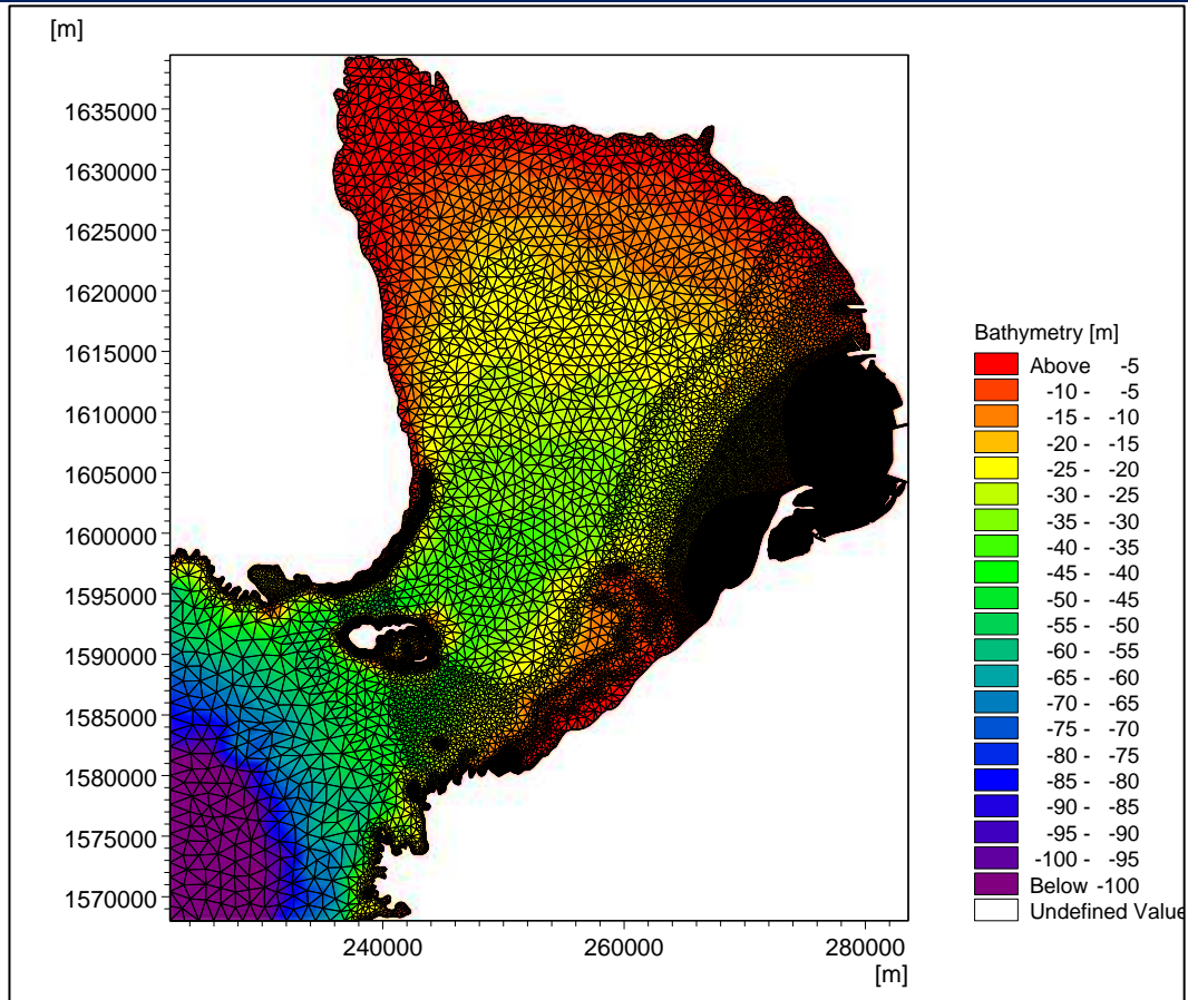
Figure 2.2-52 Flexible Element Mesh for the local Model at Manila Bay
