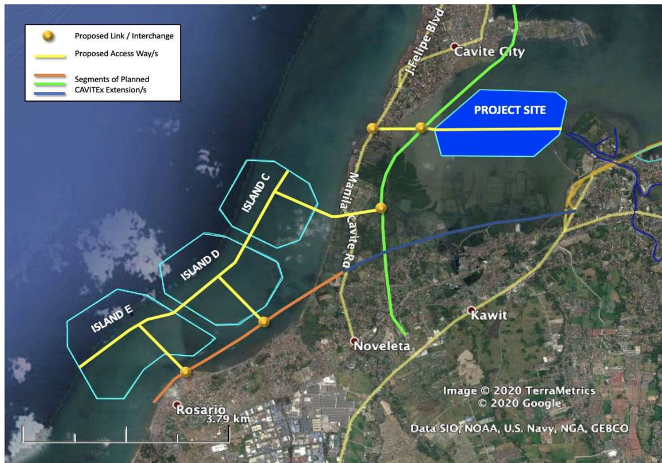
Figure 1-5. Initial Framework Plan for the Cavite Reclamation Projects Showing Conceptual Access Ways to Existing Road and the Future CAVITEx Expansion and Bridges
