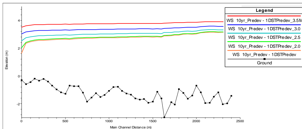
Figure 2.2-26 Imus River Profile at Various Outfall Conditions (10-year Return Period)
