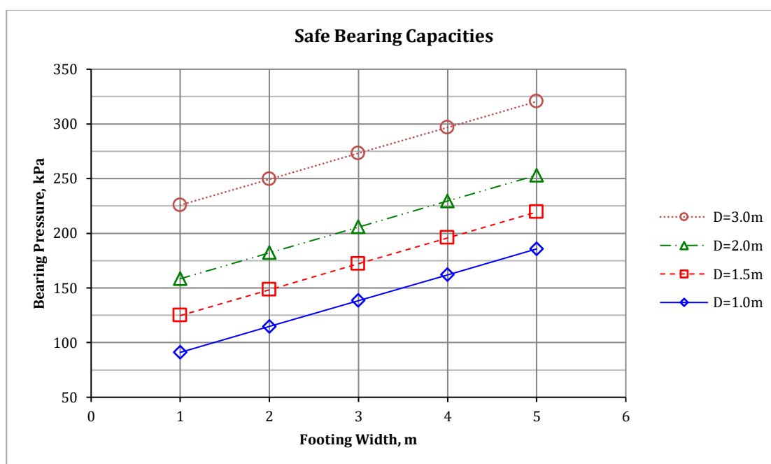
Figure 2.1-47 Safe bearing capacities for the reclamation area
