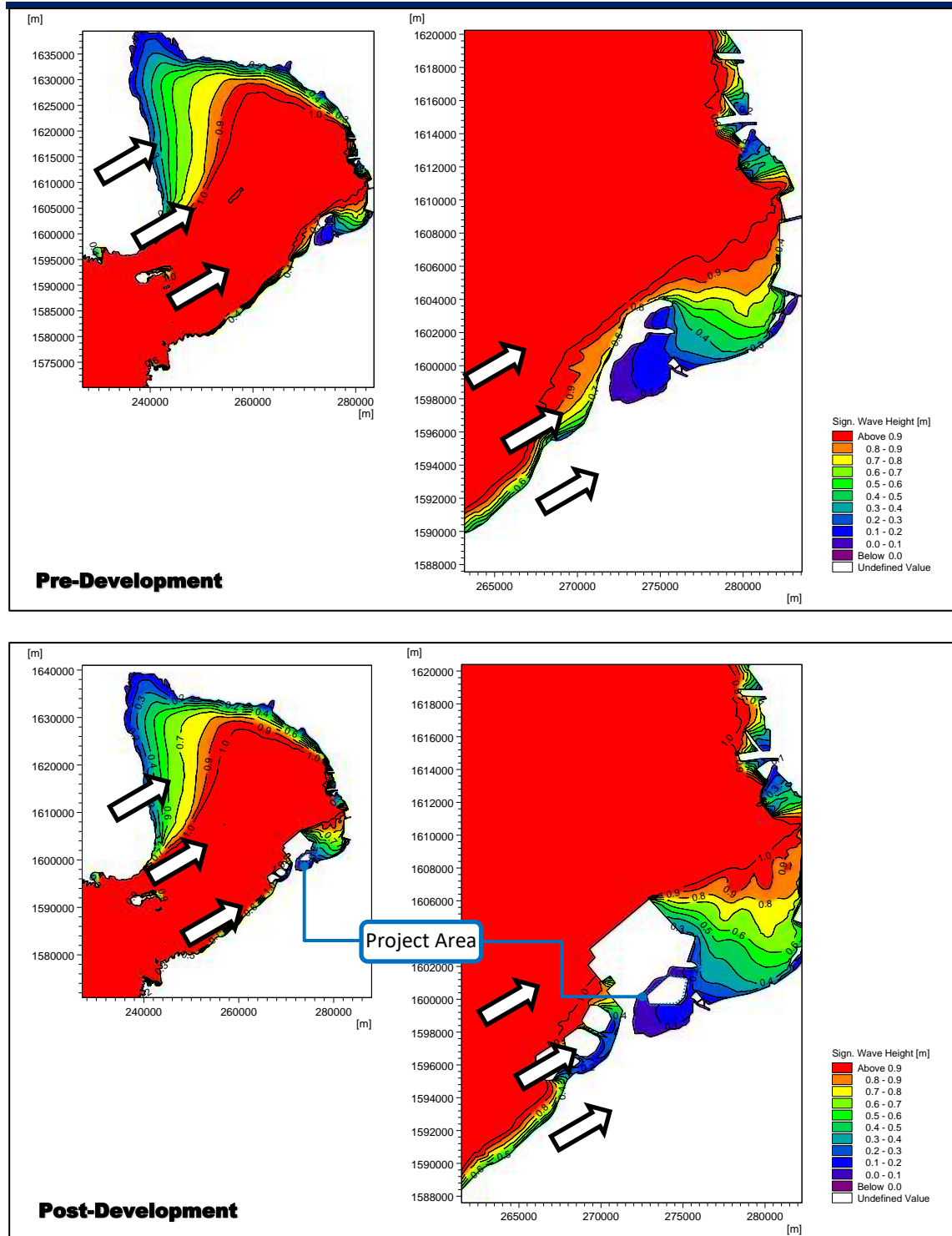
Figure 2.2-69 Wave Climate due to 9-12 mps Surface Wind & Offshore Waves from WSW at MHHW (Pre- & Post-Dev't)
