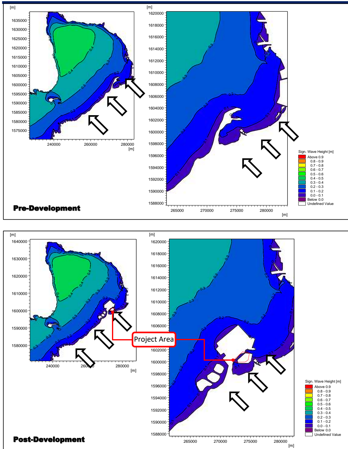
Figure 2.2-62 Wave Climate due to 1-4 mps Surface Winds & Offshore Waves from SE at MHHW (Pre- & Post-Dev't)
