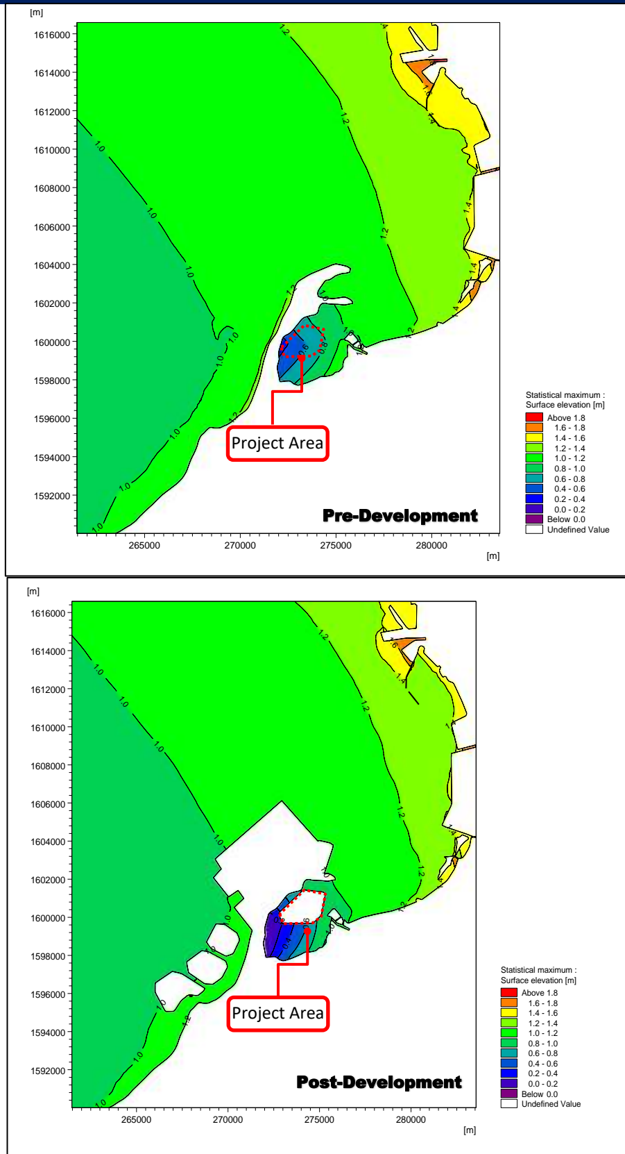
Figure 2.2-83 Simulated Storm Tide Level for Typhoon Rita/Kading (1978) Pre- & Post Development
