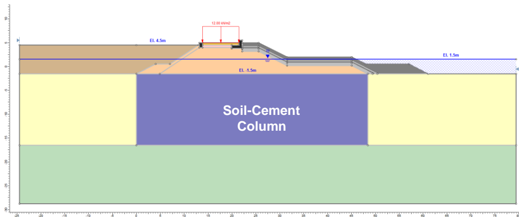
Figure 2.1-40 Slope model with soil cement column
