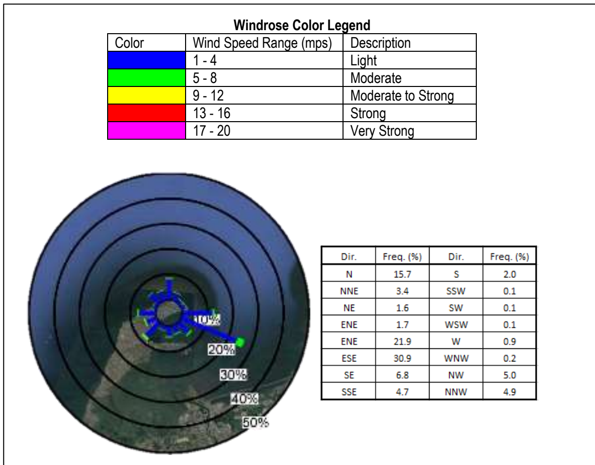
Figure 2.2-47 Annual Wind Rose Diagram at Sangley Point Station
