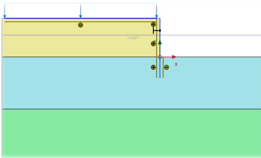
Figure 2.1-42 Plaxis Model
