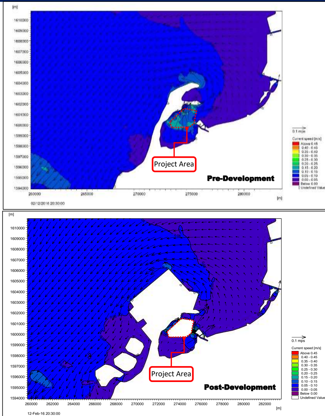
Figure 2.2-75 Snapshot of Current magnitude and direction at ebb tide (20:30 Feb. 12, 2016) Pre- & Post Development
