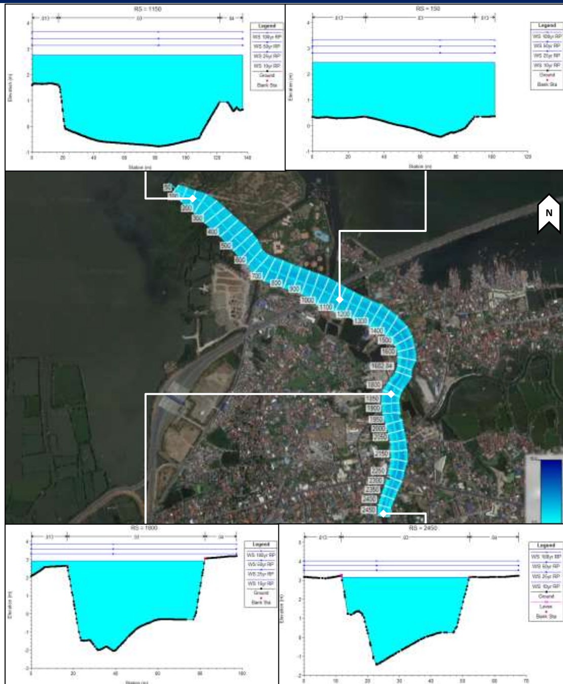
Figure 2.2-25 Sample Cross-Sections of Imus River (Pre-development and Post-development Condition)
