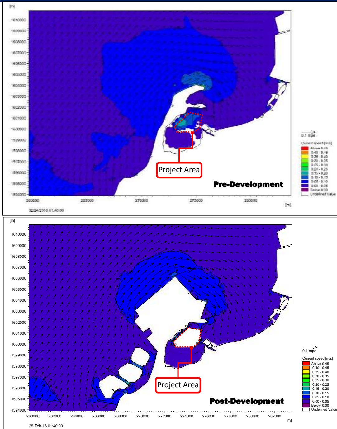
Figure 2.2-76 Current speed and direction at flow tide (01:40 Feb. 24, 2016) Pre- & Post Development
