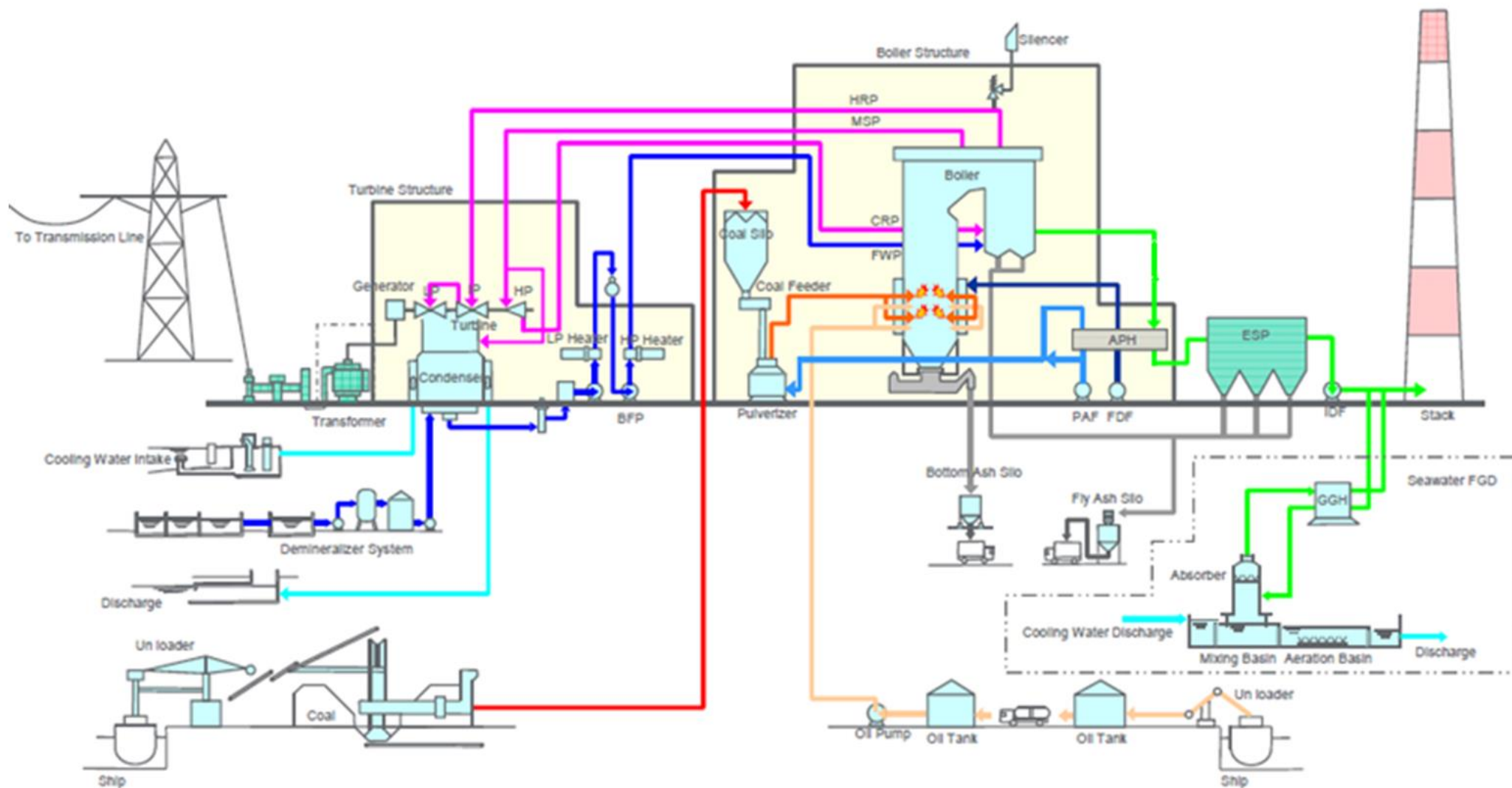
SCHEMATIC DIAGRAM OF TYPICAL COAL-FIRED BOILER PLANT
