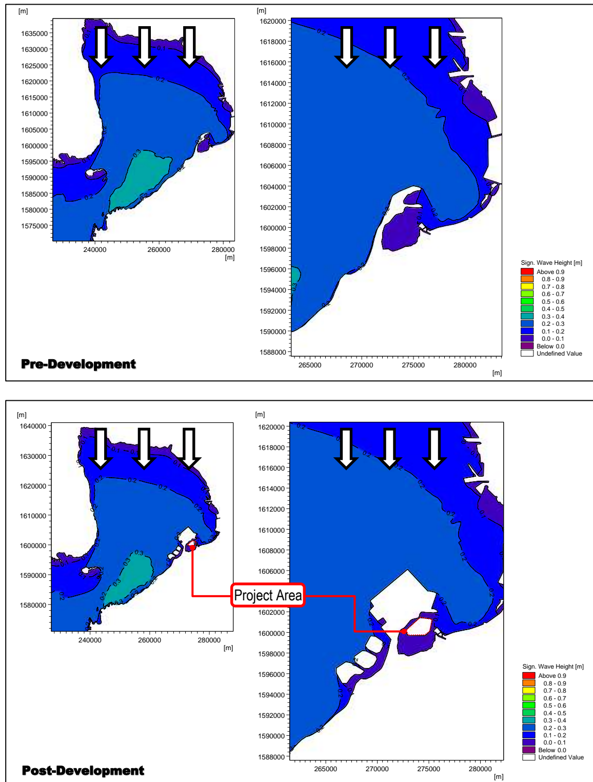
Figure 2.2-56 Wave Climate due to 1-4 mps Surface Winds and Offshore Waves from N at MHHW (Pre- & Post-Dev't)
