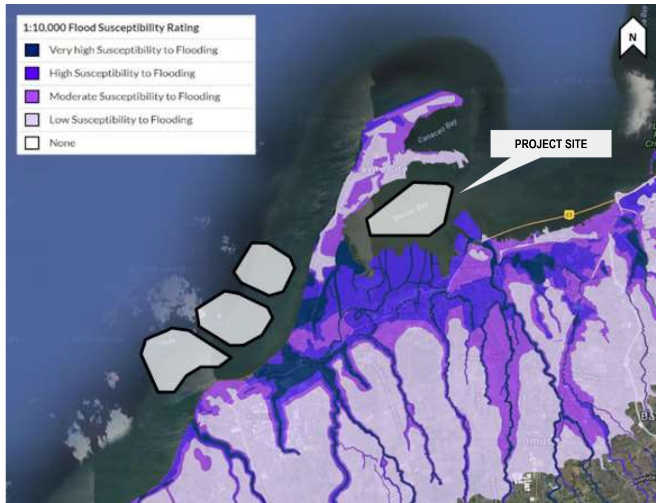
Figure 2.2-9 MGB 1:10,000 Flood Susceptibility Map
