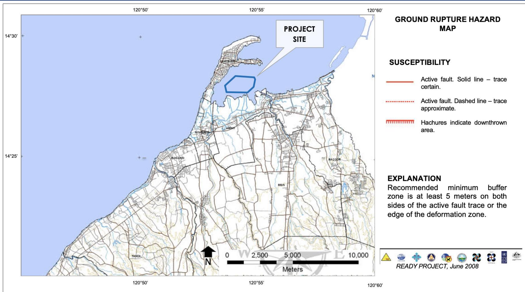
Figure 2.1-26 Ground Rupture Hazard Map of Cavite
