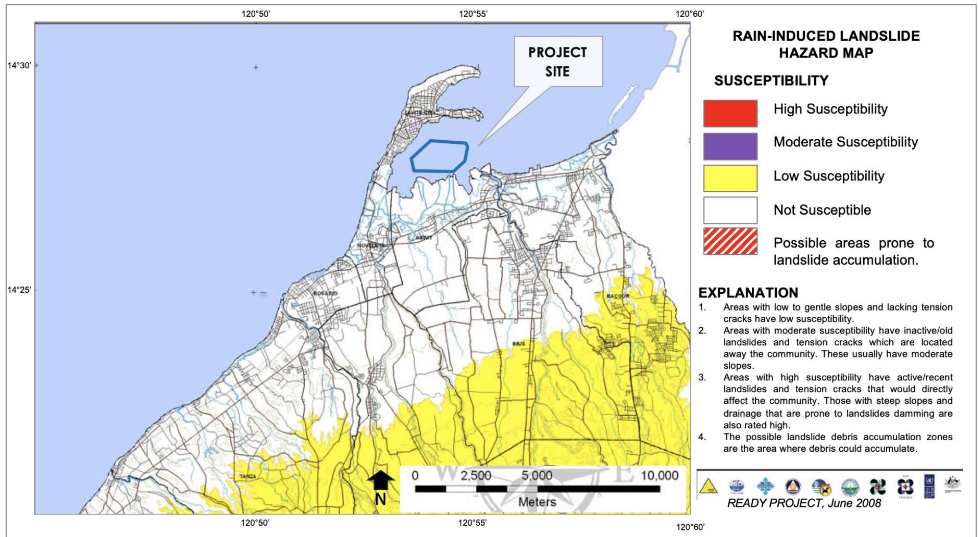
Figure 2.1-34 Rain-Induced Landslide Hazard Map of Cavite
