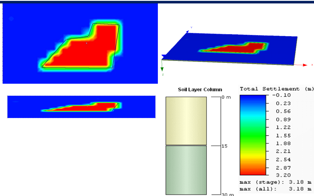
Figure 2.1-46 Settlement Analysis Results for 7m fill height
