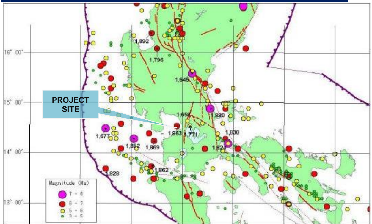
Figure 2.1-19 Distribution of Historical Earthquakes from 1608 to 1895
