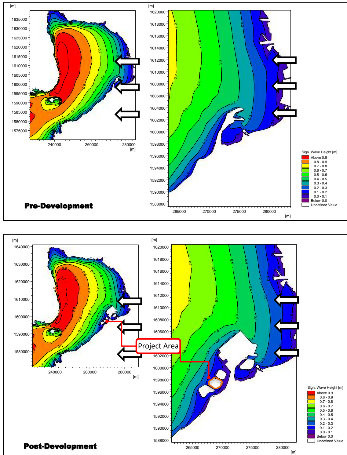
Figure 2.2-53. Wave Climate due to 5-8 mps Surface Winds & Offshore Waves from ESE at MHHW (Pre & Post-Dev.)
